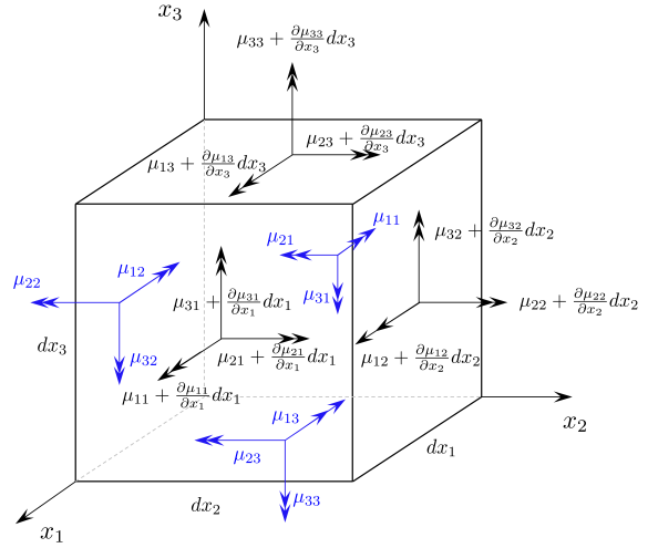
(b) Components of the couple-stress
