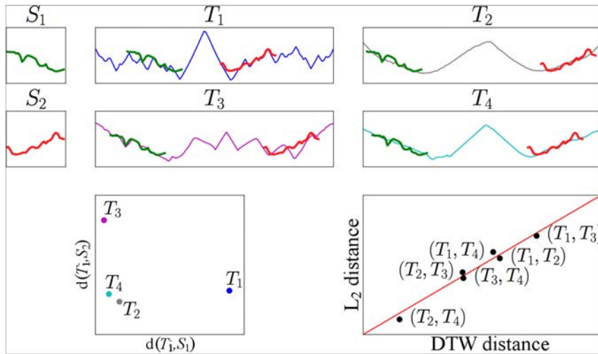
FIGURE 2.26 – Illustration of LDPS. The learned shapelets S_1 and S_2 are used to embed all TS from \mathcal{T} into a 2-dimensional space \bar{\mathcal{T}} , in which the ED is a good approximation of the true DTW measure between the pairs in the original space. In real settings, more than two shapelets are learned to obtain higher-dimensional embedding and hence richer representations. Extracted from [LMTA17].
