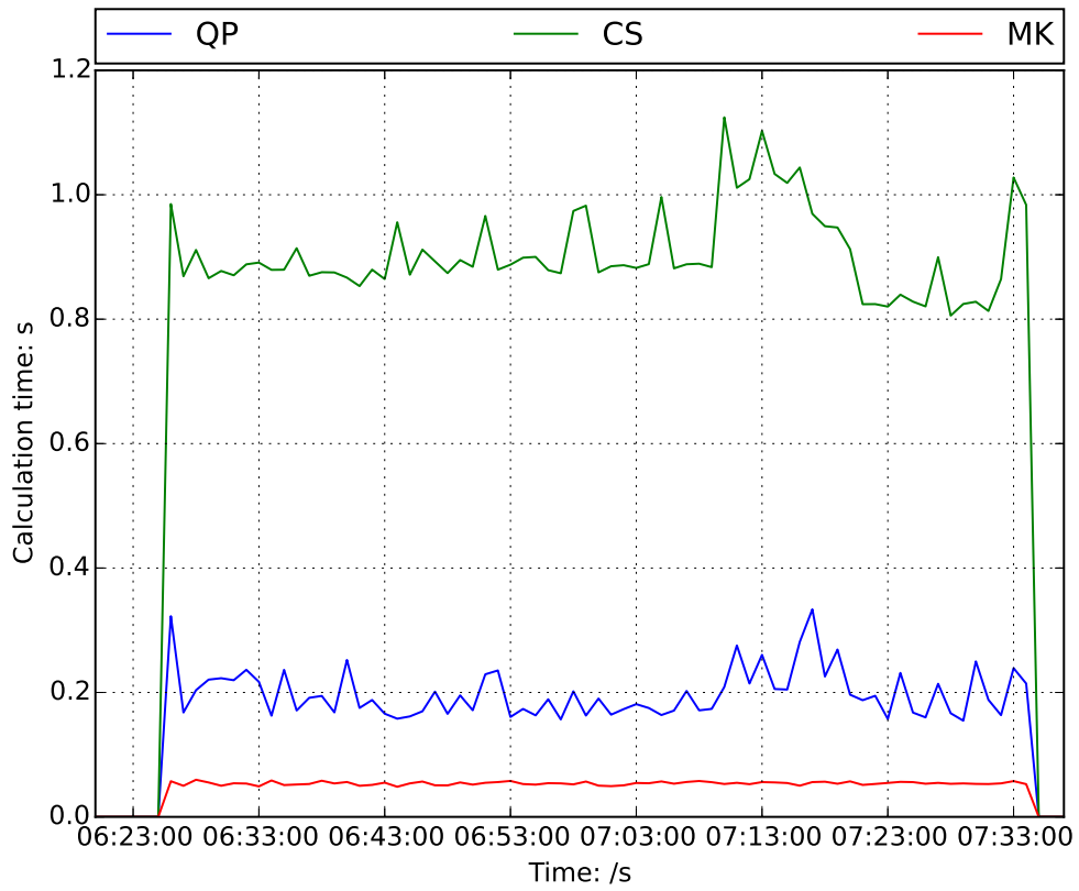
Figure 5.14: Calculation time in case 3
