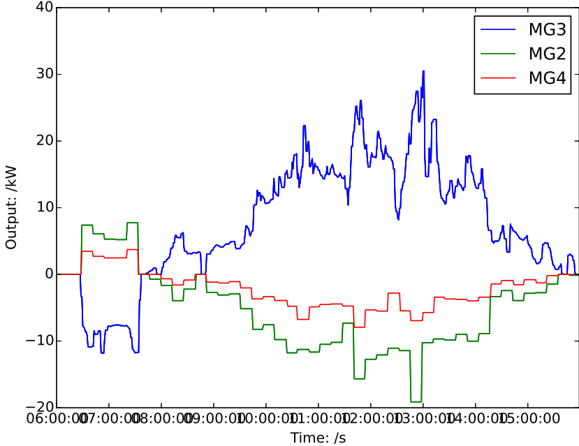
(a) MG coordinating power.
