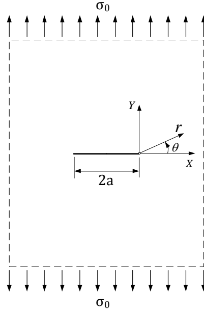
Figure 2.8: A center cracked infinite plate subjected to mode I loading (uniform tension). (Modified from [49])
