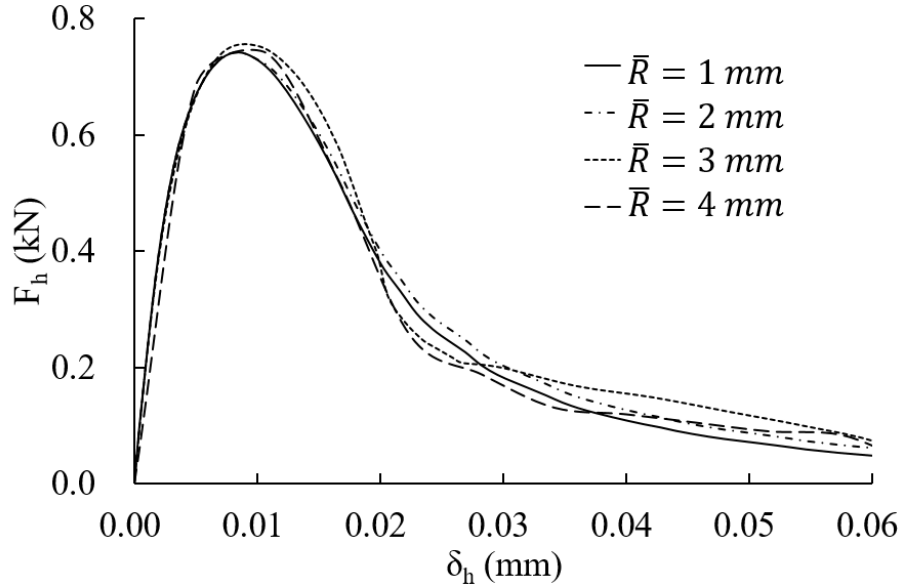
Figure 4.7: Force F_h as function of the displacement \delta_h for different particle radius.
