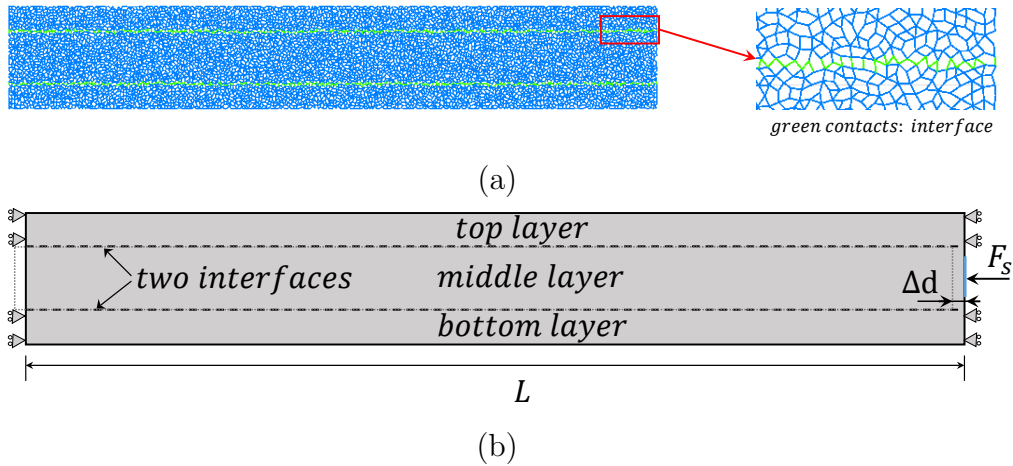
Figure 5.29: (a) Interface representation in DEM 4PB simulations. (b) Geometry of the shear test adopted in the characterisation of the interface.
