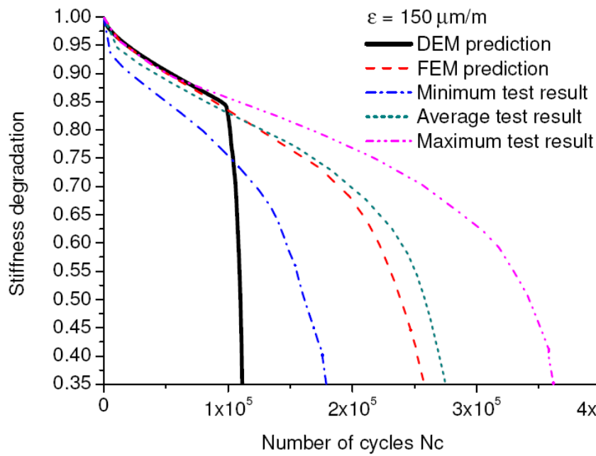
Figure 2.27: Fatigue damage curve for simulation by Gao [45], experiments FEM simulation by Arsenie [1, 16, 17].
