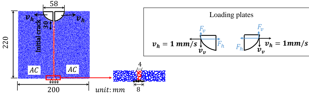
Figure 4.10: Characterization of the interface geometry on discrete element simulations.
