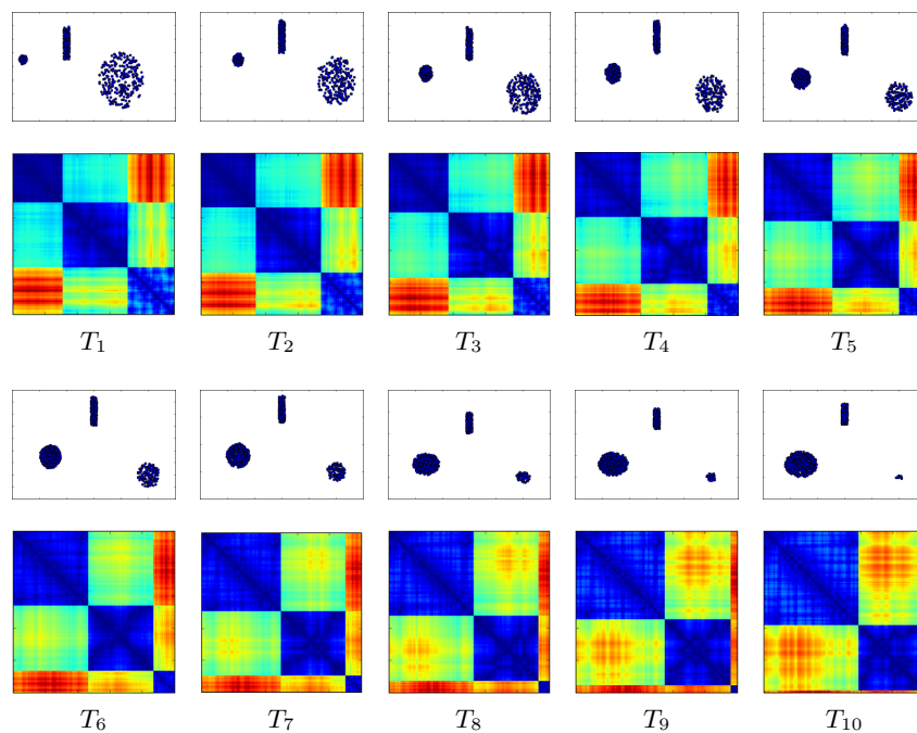
Figure 4.4: Example of visualization obtained using the proposed incremental reordering approach to the "Dyn1" data-set. The size of the matrix is kept at 1000 \times 1000 , allowing a description of the structure of the last 1000 observations.
