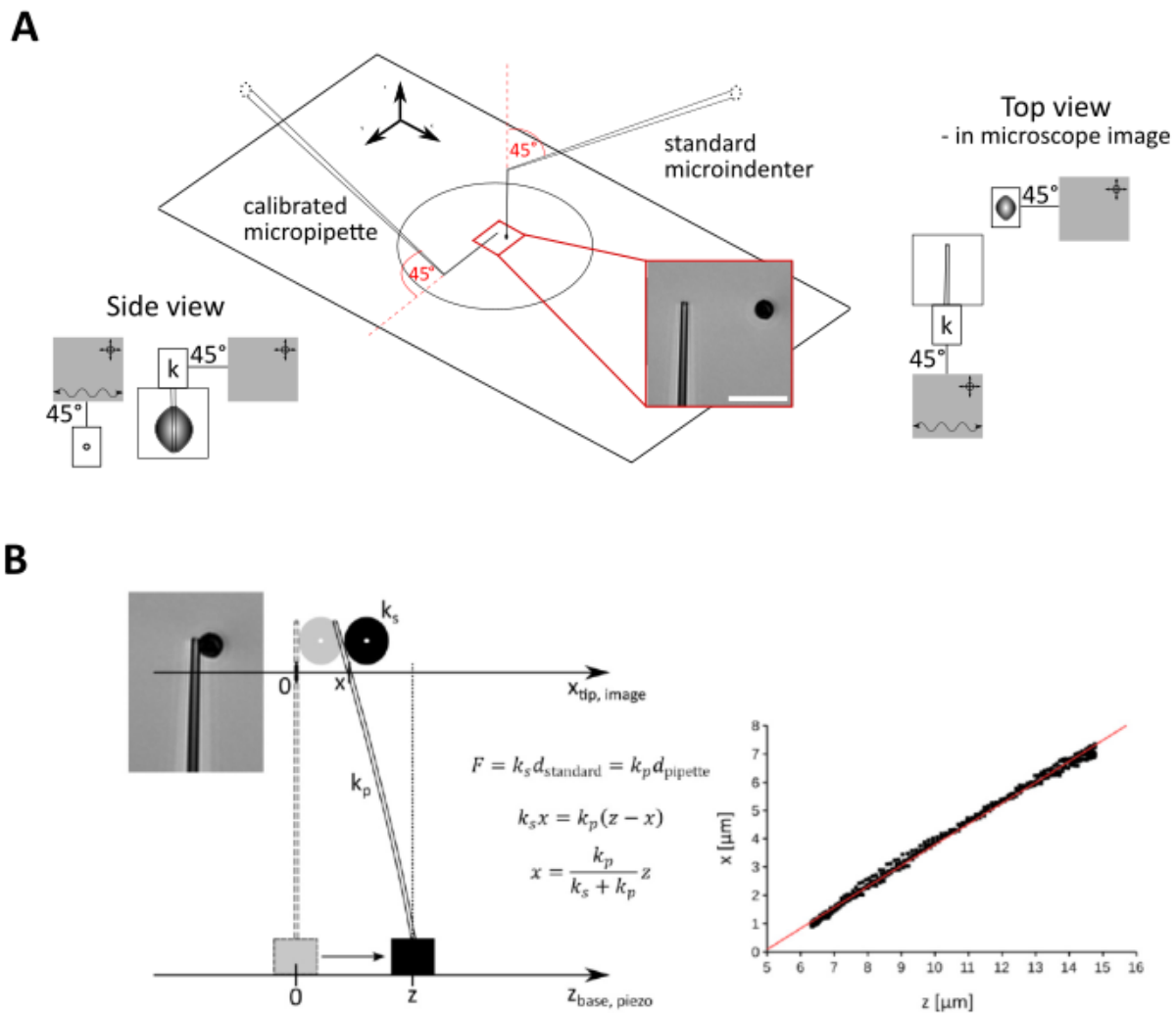
Figure 43. Micropipette calibration. A. Configuration of the micropipettes on the microscope table, drawn in 3D projection and in symbolic 2D representation, used also in Figures 14 and 16 in Chapter 1. Inset: microscope image showing a positioned micropipette and microindenter, scale bar is 20 \mu\text{m} . B. Calculation of the bending stiffness of the micropipette, k_p . The force causing the bending of the standard microindenter by a distance d_{\text{standard}} , is the same as the force causing the bending of the calibrated micropipette by a distance d_{\text{pipette}} . This equation relates the measured displacements and the bending stiffness of the micropipette and the microindenter. At each time point during calibration, the position of the tip of the micropipette ( x ) is detected in the image and plotted against the position of the base ( z ), read from the piezoelectric controller. k_p is calculated from the slope of the plot. Adapted from Supplemental Figure S8 in (Sawicka et al., 2017).
