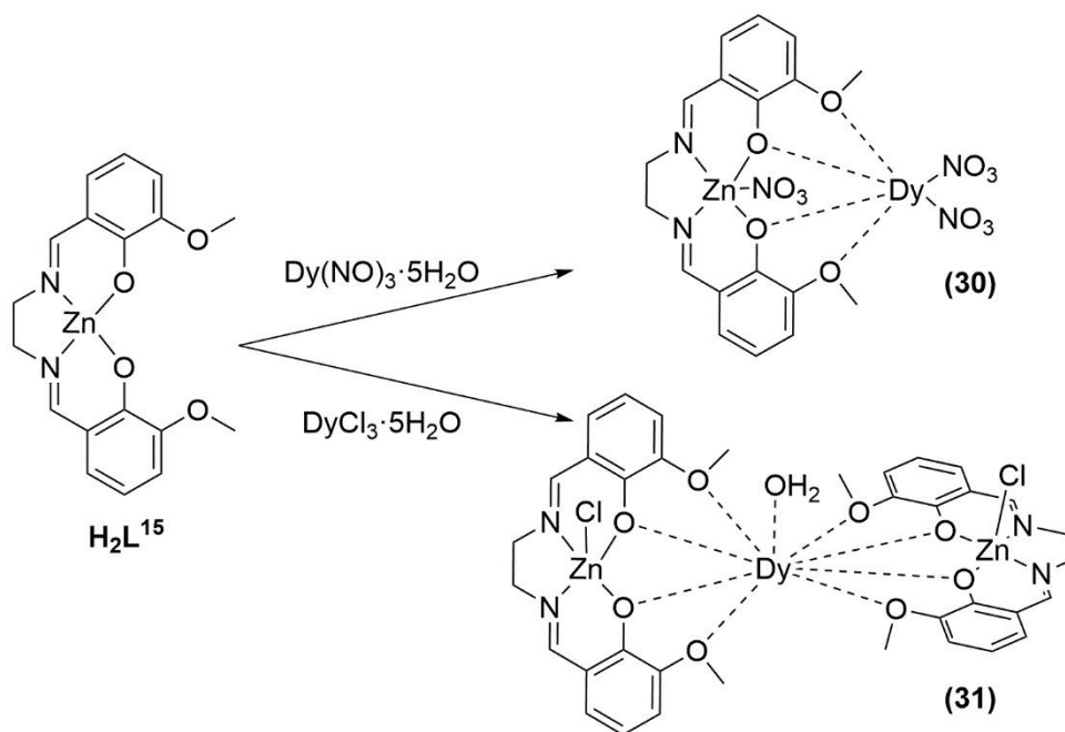
Figure 6. 1. Schema of the different routes for the formation of compounds 30 and 31 from ligand H_2L^{15} .
