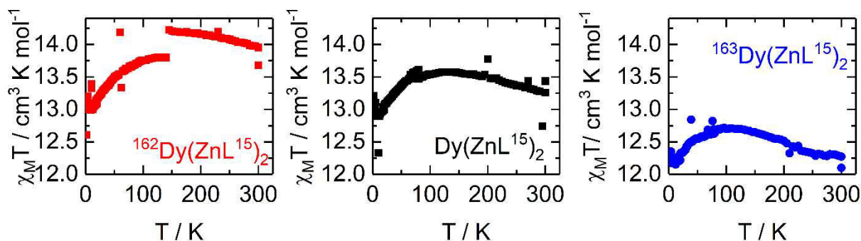
Figure A3. 1. DC magnetic susceptibility measurements of A Dy(ZnL 15 ) 2 compounds.
