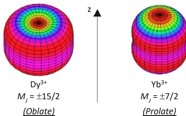
Figure 1. 6. Representation of two different examples of the categories of Lanthanides depending on their electronic density shape: oblate ( \text{Dy}^{3+} ) or prolate ( \text{Yb}^{3+} ).
