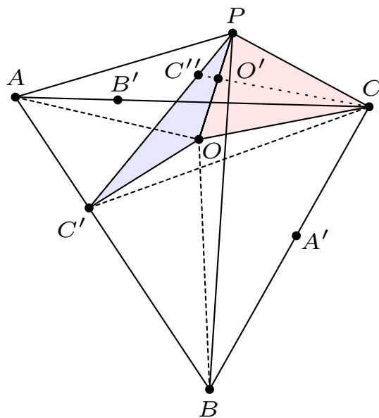
FIGURE III.2.13 – Illustration de la preuve du lemme III.2.8.
