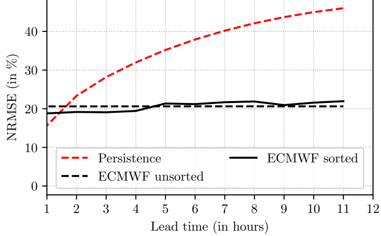
Figure 2.1 | Comparison of ECMWF performances when t_0 refers to 00:00 UTC or 12:00 UTC ('ECMWF sorted') and when t_0 refers to the starting time of the downscaling models forecasts ('ECMWF unsorted'). In the first case, there are two forecasts a day (00:00 UTC or 12:00 UTC), in the second cases these are hourly forecasts. The performance of persistence (described in 2.2.3) is added as reference.
