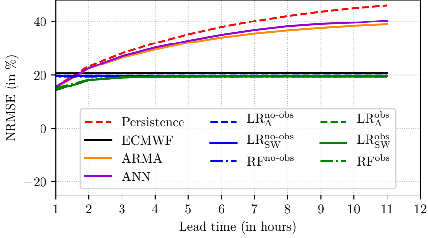
Figure 2.7 | Performances of downscaling statistical models for hourly forecasts from 1 h to 11 h in two configurations against the performances of ECMWF and the benchmark method. LR_A^{no-obs} , LR_{SW}^{no-obs} , and RF^{no-obs} display the downscaling of explanatory variables from ECMWF outputs only. LR_A^{obs} , LR_{SW}^{obs} , and RF^{obs} show the results when the error between the measurements at t_0 and the 100-m wind speed forecasted by ECMWF at t is adding as explanatory variable. Results of persistence, ANN, and ARMA are added.
