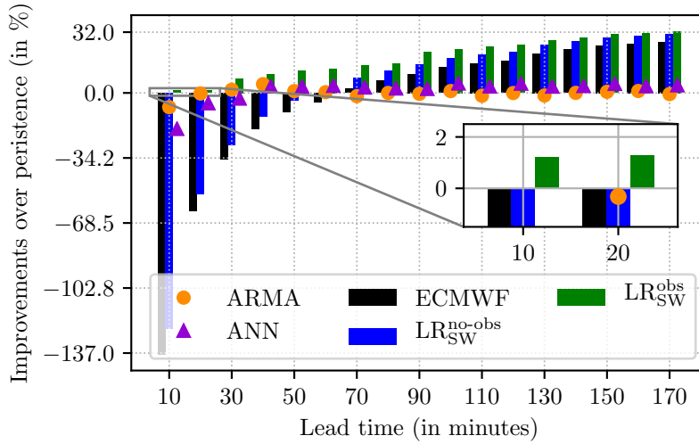
Figure 3.18 | Comparison of the improvements over persistence in percentage for ECMWF forecasts and the best downscaling models: LR_{SW}^{obs} and LR_{SW}^{no-obs} from 10 min to 170 min. Improvements of ECMWF, ARMA, and ANN methods are also included. In every case, the downscaling model is used to forecast the wind speed, and the wind power is retrieved using the power curve.
