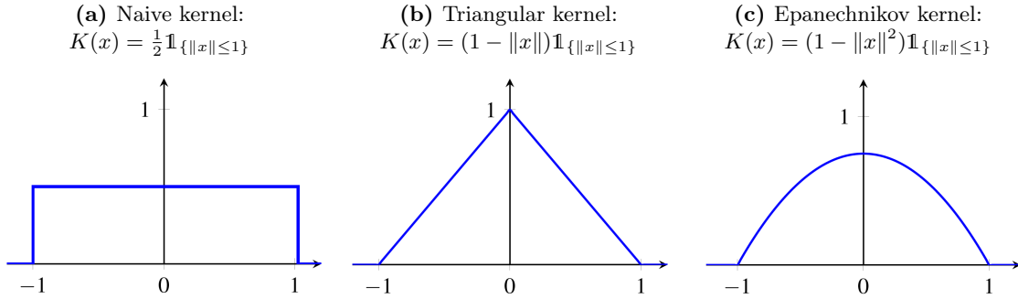
Figure A.1 | Some examples of normalized kernel functions K .
