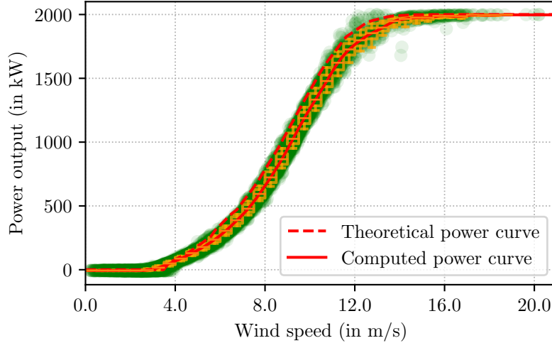
Figure 3.2 | Computed power curve for the turbines at Parc de Bonneval. For each 0.5 \text{ m s}^{-1} interval, the boxplots of the distribution are shown in orange. The whiskers correspond to the first and the ninth deciles. The means of each interval are fitted in order to retrieve the power curve. The theoretical power curve provided by the turbine manufacturer is also shown by the dashed line.
