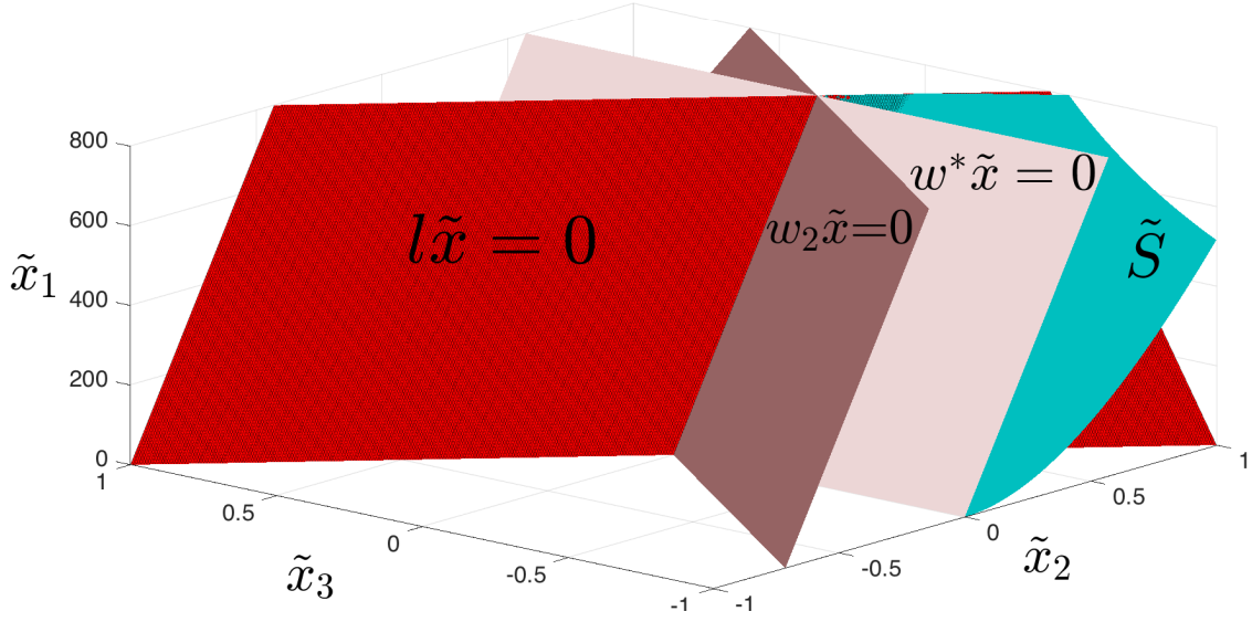
Figure 6.1 The largest polyhedral PIS in open-loop using IF2 patient parameters. The largest Polyhedral PIS \Omega(G^*) is with w = w^* . The plane w_2 \tilde{x} = 0 is with c = 1000 to characterize \Omega(G_2) .
