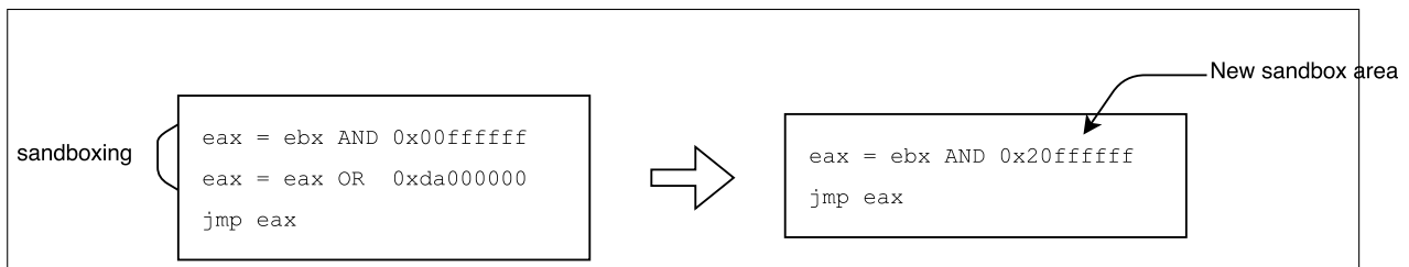
Figure 1.9 – Reducing the sandboxing to a single instruction
