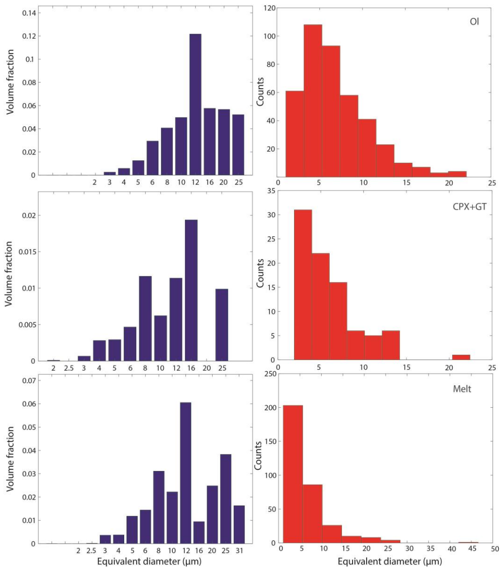
Figure B.18 Grain size and volume fraction as a function of grain equivalent diameter of all computed FOAMS images for each phase on M490. Cpx and Gt are treated together due to similar color in BSE microphotographs.
