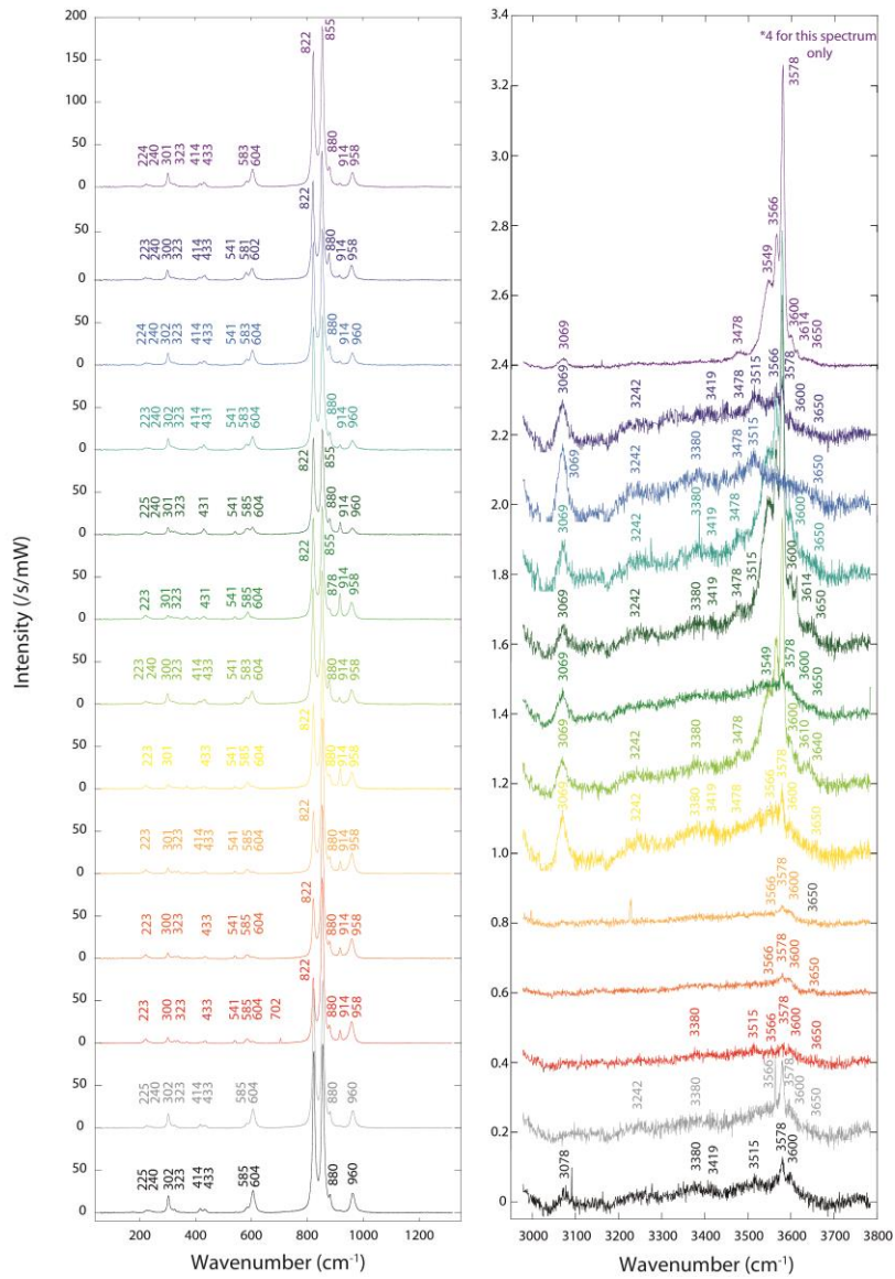
Figure A.13 Raman analyses of M525. On the left panel silicate region is represented. On the right panel the OH frequency region is given.
