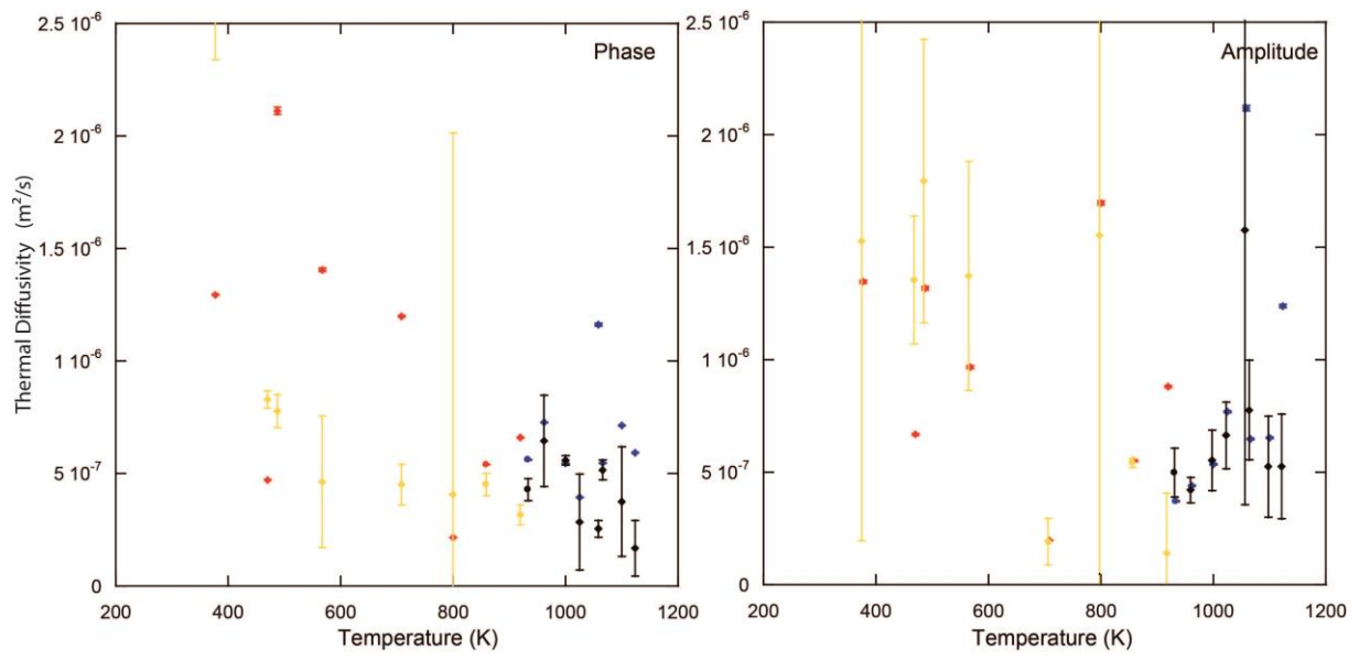
Figure D.52 M808 Thermal diffusivities obtained after fitting ( D_0 ) and average (AVG) methods on diffusivities obtained at different frequencies at a fixed temperature. Phase and amplitude thermal diffusivity estimations are given in left and right panels respectively.
