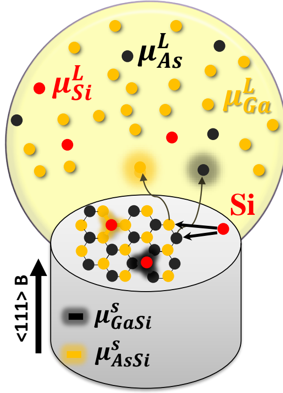
Figure II.5: Illustration of the VLS growth of \langle 111 \rangle -B-oriented zinc-blende GaAs NWs with Si, which can be incorporated into either Ga or As sites of GaAs. Replacing Ga with a Si atom (n-type doping) creates As-Si pair with a contribution \epsilon_{AsSi} to the total internal energy and increases the chemical potential \mu_{Ga}^L by adding one Ga atom to the liquid. Replacing As with a Si atom (p-type doping) creates Ga-Si pair with a contribution \epsilon_{GaSi} to the total internal energy and increases the chemical potential \mu_{As}^L by adding one As atom to the liquid.
