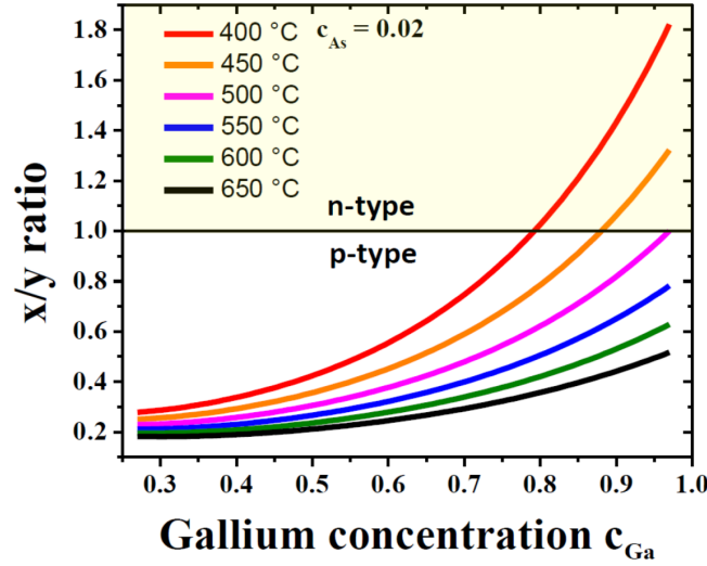
Figure II.8: The ratio x/y versus c_{Ga} at a fixed c_{As} = 0.02 and different MBE growth temperatures, showing the tendency for n-type doping at lower temperatures.
