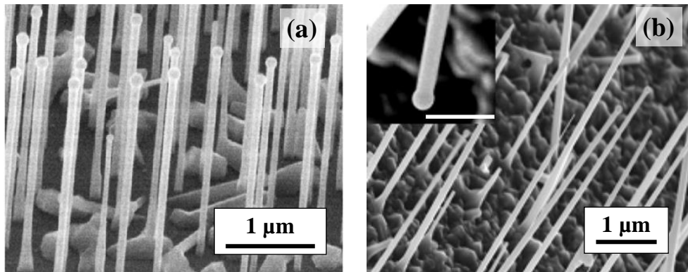
Figure I.3: Scanning electron micrographs of MBE grown GaAs NWs obtained by (a) Colombo et al. on a (111)B GaAs substrate sputtered with a 10 nm \text{SiO}_2 layer [31], and (b) Jabeen et al. on Si(100) cleaved wafers [32]. The inset (scale bar 200 nm) shows a detail on the final end of a selected NW.
