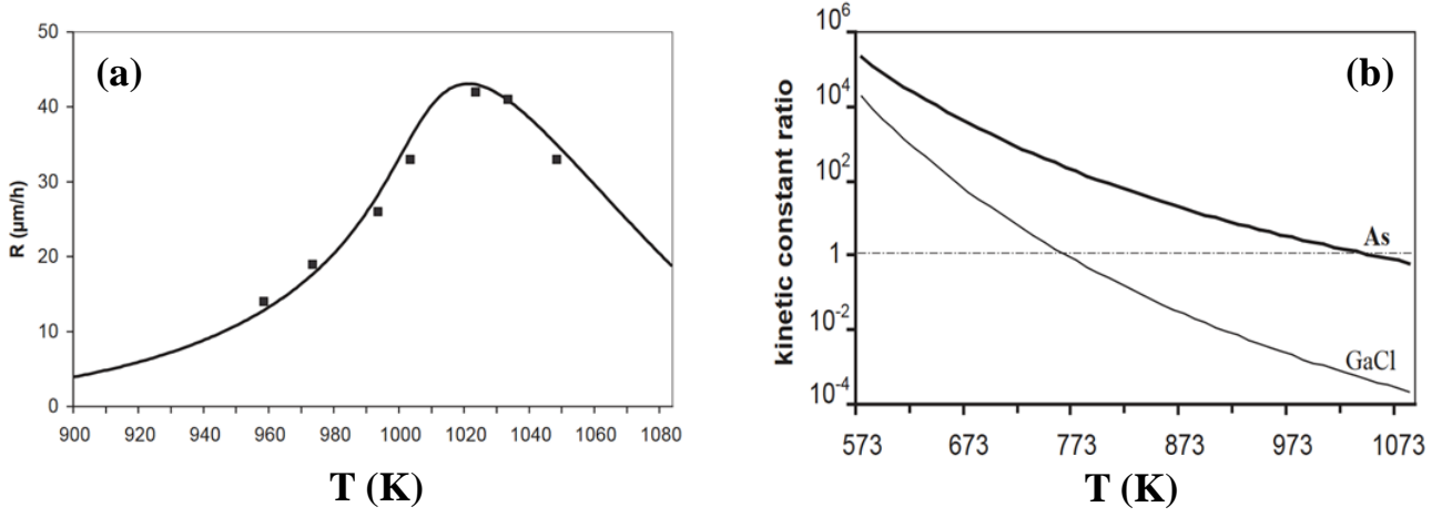
Figure I.8: (a) (001) GaAs growth rate R in \mu\text{m/h} as a function of the temperature T for standard experimental conditions ( \text{III/V} = 4.5 , \gamma = 4 ). The squares are the experimental points; the full line is the computed theoretical curve according to the modeling described in Ref. [50]. (b) Variations of the adsorption/desorption kinetic constant ratio k_{+i}/k_{-i} for GaCl (thin solid line) and As (thick solid line) as a function of T . The kinetic constants are part of the adsorption J_{ads} = k_{+i}\theta_{vacant} and desorption J_{des} = k_{-i}[i]\theta_i fluxes of species i = \text{GaCl} or As, with [i] being the partial pressure of gaseous species i , \theta_{vacant} the surface coverage ratio in vacant sites, and \theta_i the surface coverage ratio of ad-species i . The k_{+i}/k_{-i} ratio gives the contribution of the microscopic states involved in the dynamic surface-vapor system [50]. The actual J_{ads}/J_{des} ratio should include the input mass of species i ( [i] ), which ensures sufficient adsorption of GaCl up to 1040 K.
