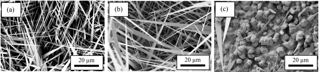
Figure II.2: Scanning electron microscopy (SEM) images of GaAs structures grown at 715 °C after depositing 1 nm of gold on Si(111) (a) with 500 nm of thermal SiO 2 , (b) native SiO 2 and (c) without SiO 2 . These images were taken in InLens mode with an electronic incident energy of 3 KV.
