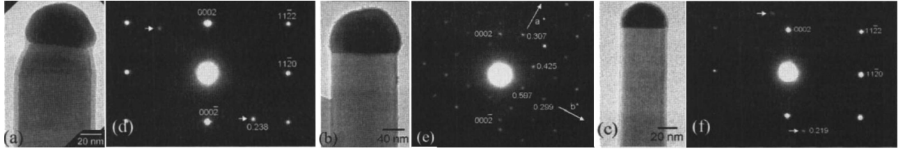
Figure I.2: HR-TEM views showing the ends of three types of NWs after growth at 630^\circ\text{C} : (a) NW A: 45 min of growth, the Ga flux was stopped at the end of growth while \text{As}_2 was maintained for 2 min at 590^\circ\text{C} ; (b) NW B: 45 min of growth, the Ga and \text{As}_2 were stopped simultaneously before cooling down the substrate; and (c) NW C: the same termination of B except the growth time was 160 min. (d), (e) and (f) are the corresponding electron diffraction patterns of droplets A, B and C, respectively. [22]
