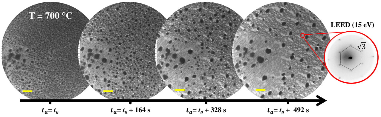
Figure I.11: LEEM images ( E = 1.8 eV) showing the evolution of the Au-Si clusters diffusing on the surface while decomposing the native \text{SiO}_2 at 700 °C. The effective thickness of Au is 1 nm, deposited at RT before annealing. The yellow bar represents 1 \mu\text{m} . At the right, a LEED pattern of the trace formed behind the diffusing cluster is shown. The dashed hexagon evidences that the unveiled surface exhibits a \sqrt{3} \times \sqrt{3} reconstruction.
