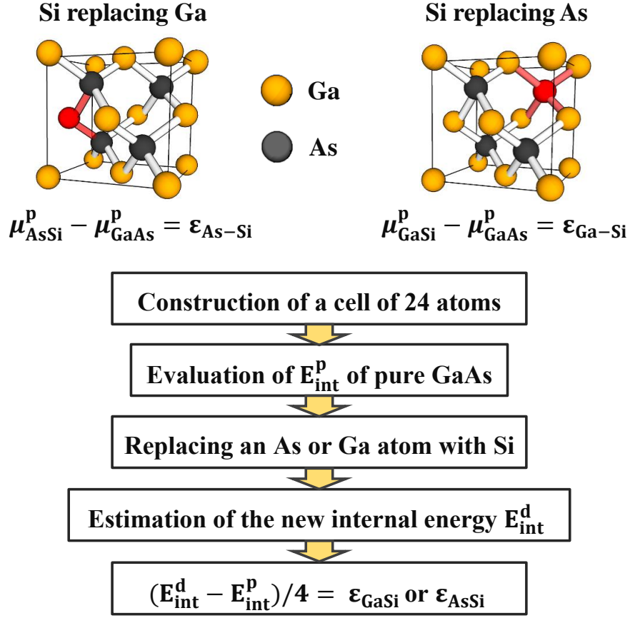
Figure II.6: Diagram showing different steps used for calculating the energy contributions \epsilon_{\text{GaSi}} and \epsilon_{\text{AsSi}} by DFT.
