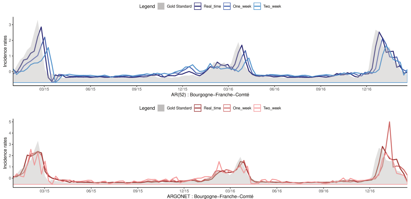
Figure S3. Evolution of Bourgogne-Franche-Comté estimates over time for AR(52) and ARGONET models
