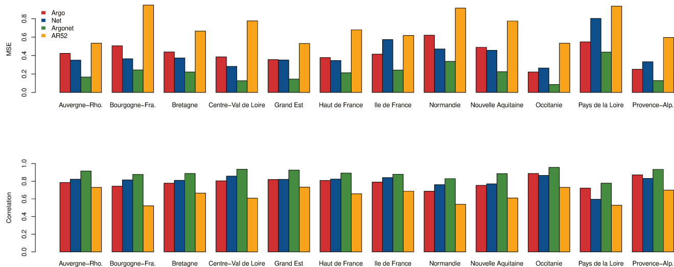
Figure 11. PCC and MSE obtained for two-week forecast with ARGO, Net and ARGONet models
