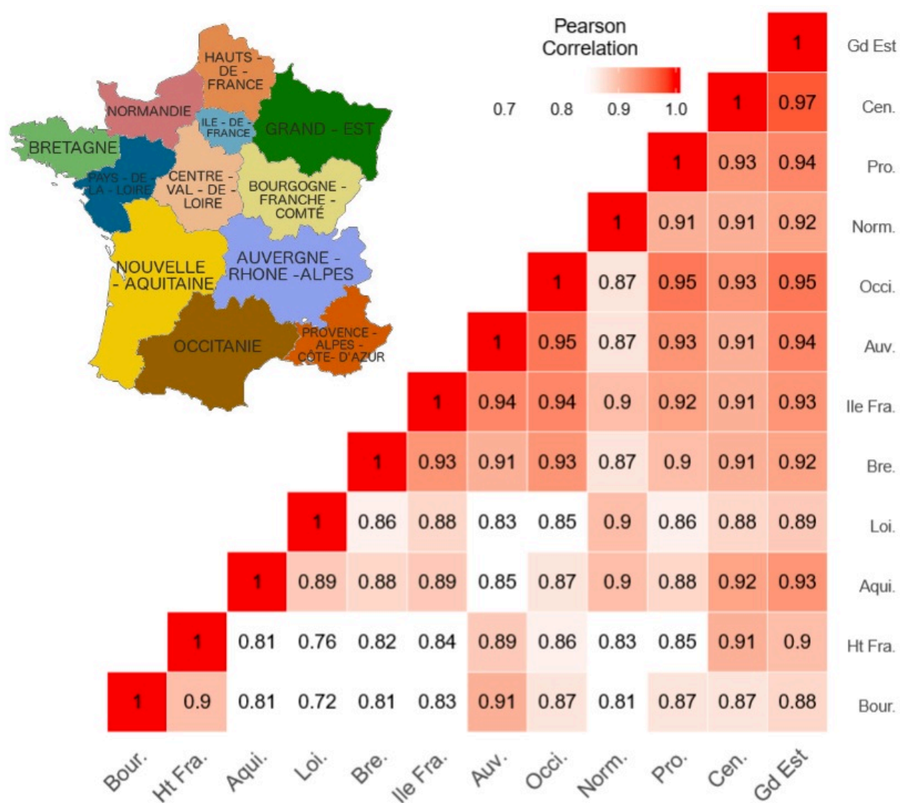
Figure S1. Correlation between French regions on the period starting from January 2013 to March 2017
