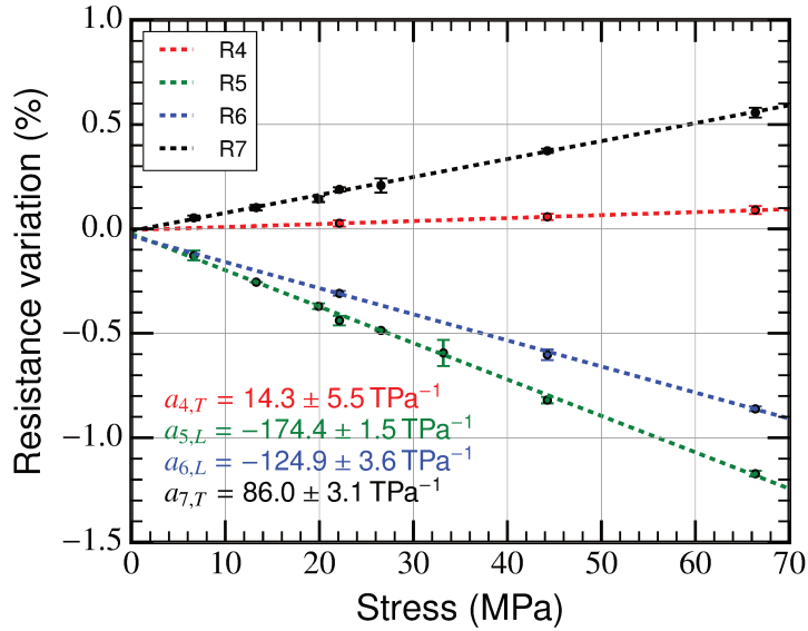
FIGURE IV.12: Relative resistance variation as a function of prescribed stress during the calibration procedure by four-point bending for N-type resistors (mean \pm 3 \times SE).
