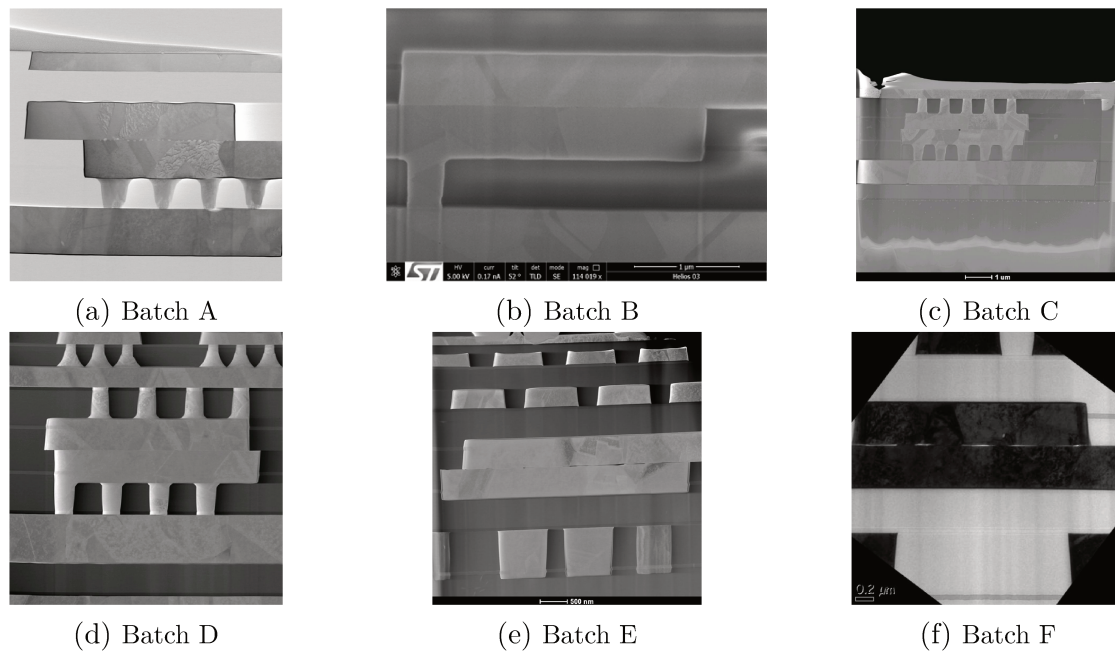
FIGURE II.6: FIB cross-sections of the Cu-Cu interface between pads of width 4.4\ \mu\text{m} after post-bonding annealing for wafers having undergone various CMP processes, with increasing selectivity: (a) scanning TEM; (b) SEM; (c)-(e) scanning TEM; (f) energy-filtered TEM
