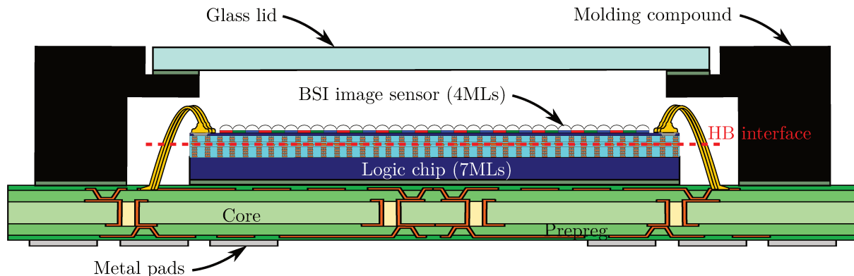
FIGURE I.30: Schematical description of the 3D image sensor studied in this work.
