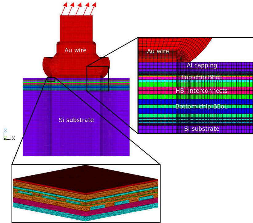
FIGURE III.6: Global and local finite element models used in the multi-scale approach for simulating the wire pull test (with zoomed view on the homogenized layers of the BEoL in the global model).
