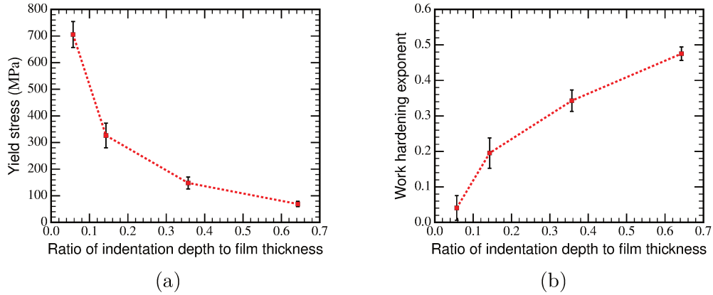
FIGURE B.3: (a) Yield stress and (b) work hardening exponent of the Cu thin film, obtained as a function of indentation depth from the reverse analysis methodology of Dao et al. [7].
