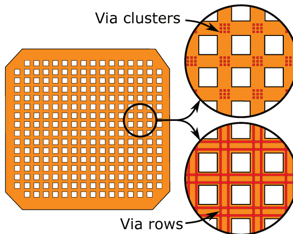
FIGURE III.4: Schematic description of the two types of patterning introduced for the via levels in-between crossing metal lines (for example here in the “grid” configuration).
