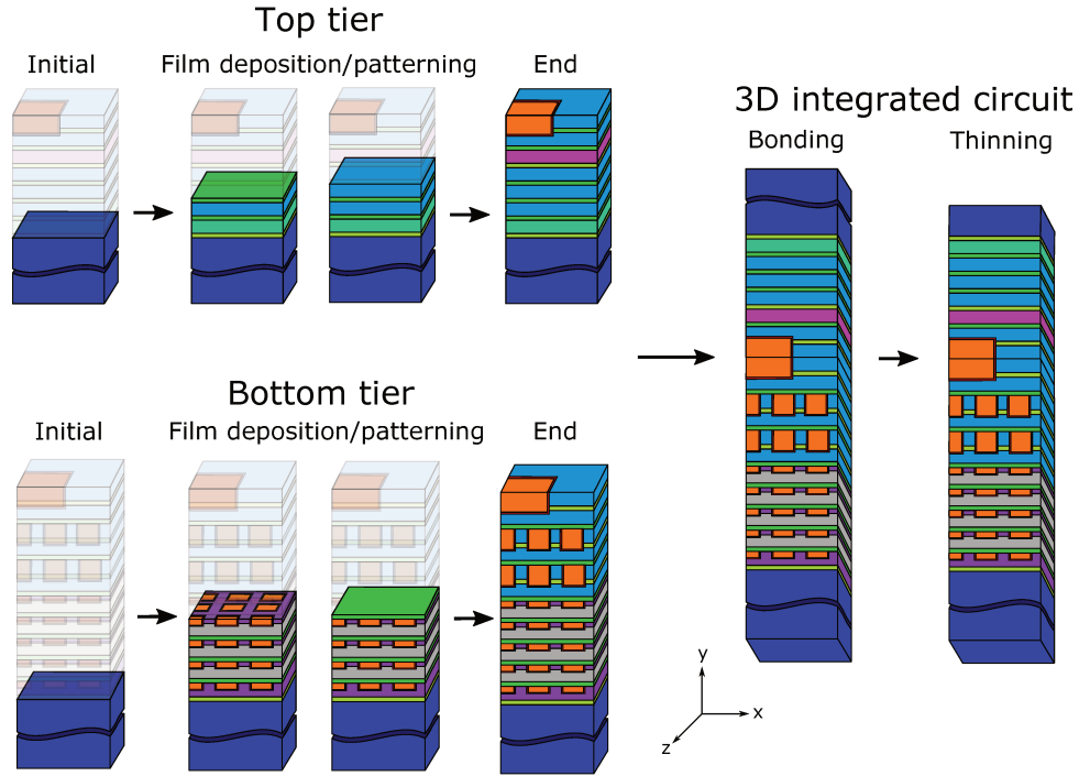
FIGURE IV.21: Schematical description of the different steps in the finite element analysis to account for the whole front-end process sequence.
