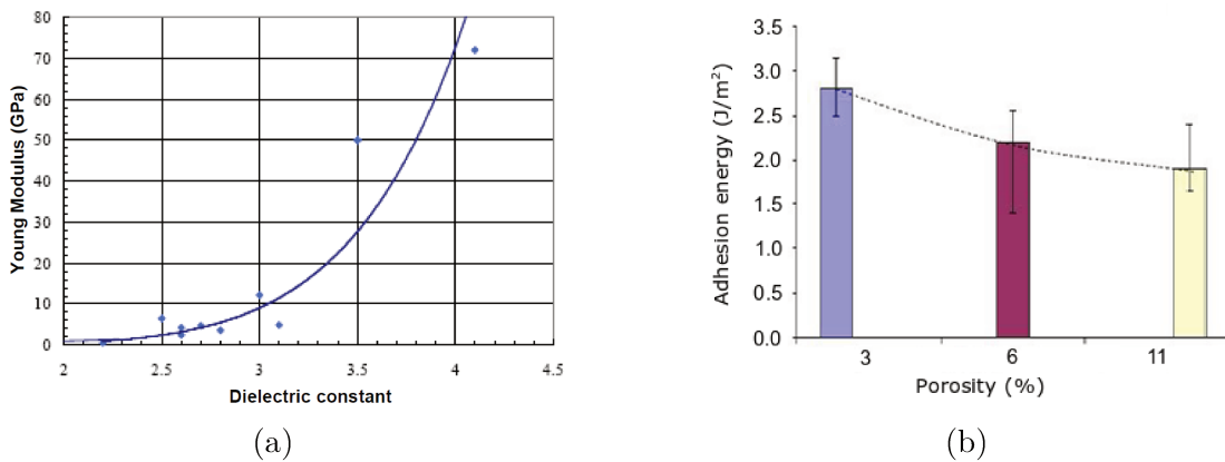
FIGURE I.12: Graphs illustrating (a) the decrease in the Young's modulus of low-k and ultra-low-k dielectric materials [19], and (b) the influence of ultra-low-k dielectric porosity on the adhesion energy of a SiOC:H/USG interface [20].
