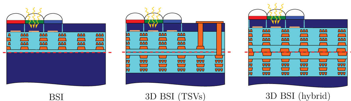
FIGURE I.29: Schematical comparison between the dual- TSV and hybrid bonding approaches for 3D stacking of image sensors.
