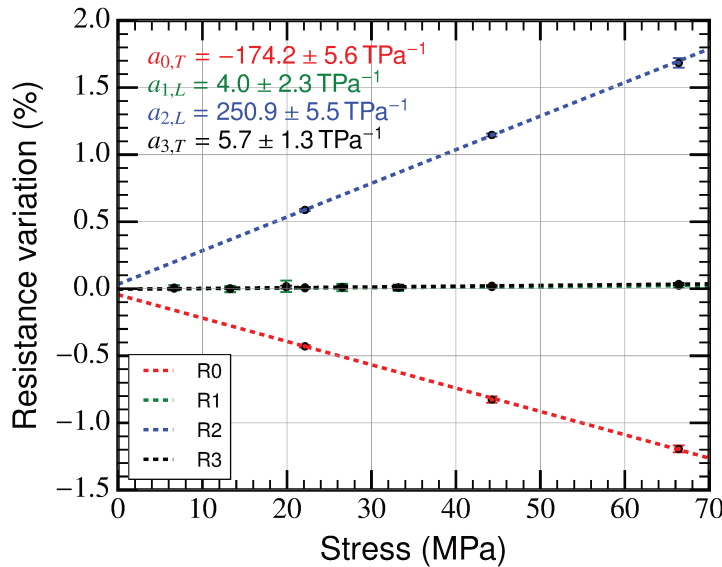
FIGURE IV.11: Relative resistance variation as a function of prescribed stress during the calibration procedure by four-point bending for P-type resistors (mean ± 3 × SE).
