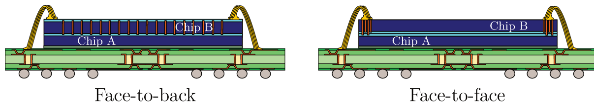
FIGURE I.28: Schematical comparison between the F2B and F2F approaches [54].
