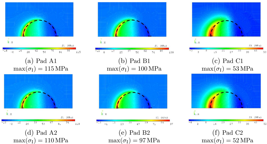
FIGURE III.14: Contour plots of the 1 st principal stress in the homogenized CO layer for the studied pad structures (top view). The black dotted half-circle marks the wire bond footprint.
