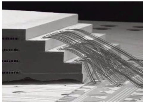
FIGURE I.25: Tilted SEM view of a system-in-package formed by vertical chip stacking using wire-bonding assembly [48].
