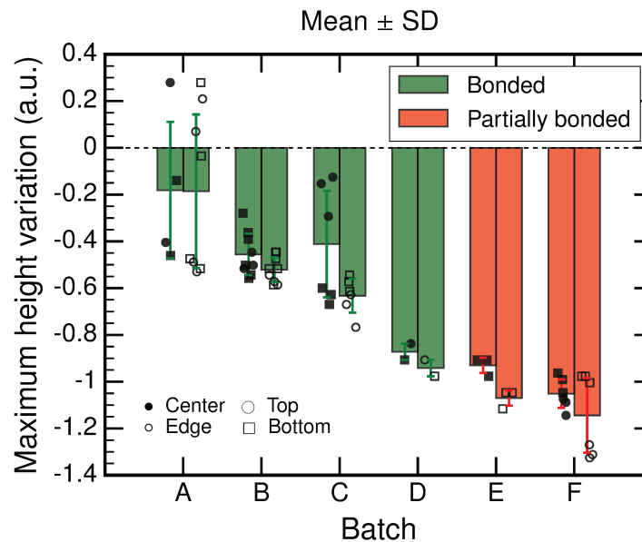
FIGURE II.8: Comparison of hybrid bonding pad surface topography measured on several sites by AFM with bonding quality evaluated qualitatively from FIB/SEM cross-sections on wafers extracted from the same lot.
