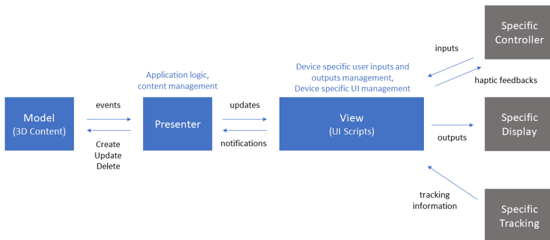
FIGURE 2.2 – Application des principes de Model-View-Presenter aux applications 3D
