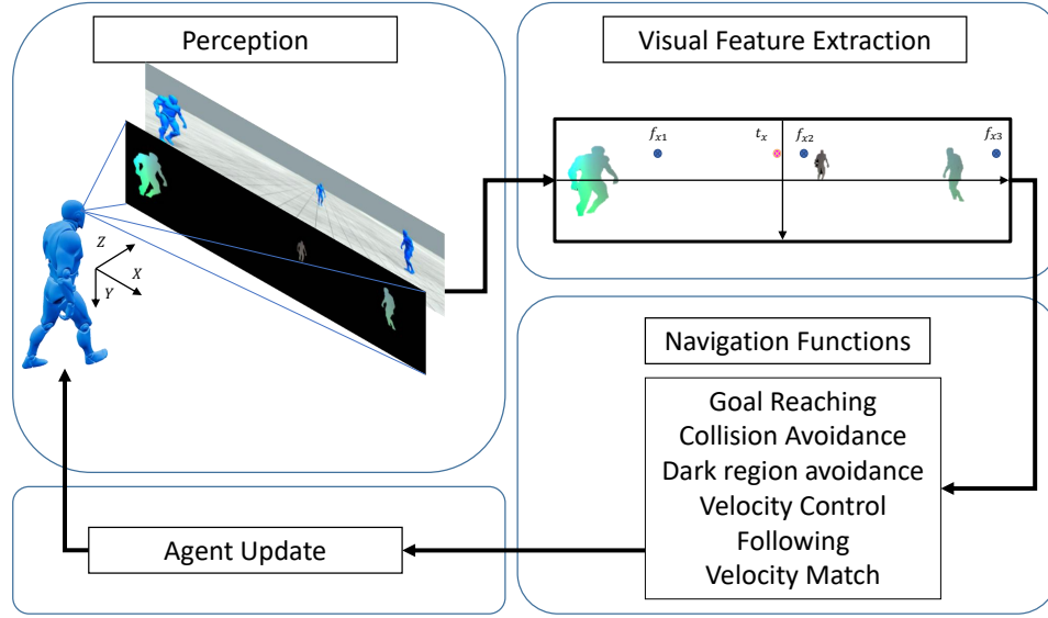
Figure 10 – Illustration of the 4 stages of the vision-based control loop for character navigation.
