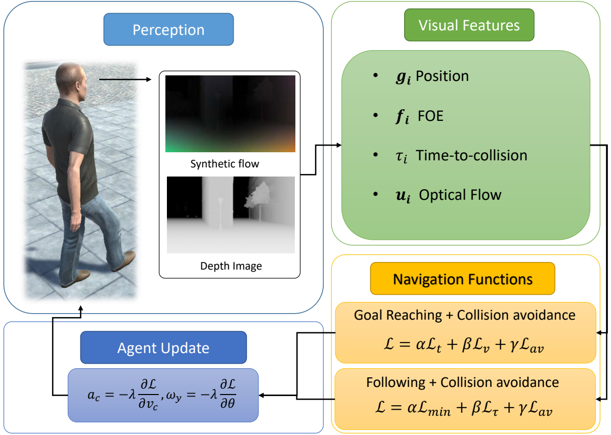
Figure 3.6 – Agent control loop using synthetic optical flow.
