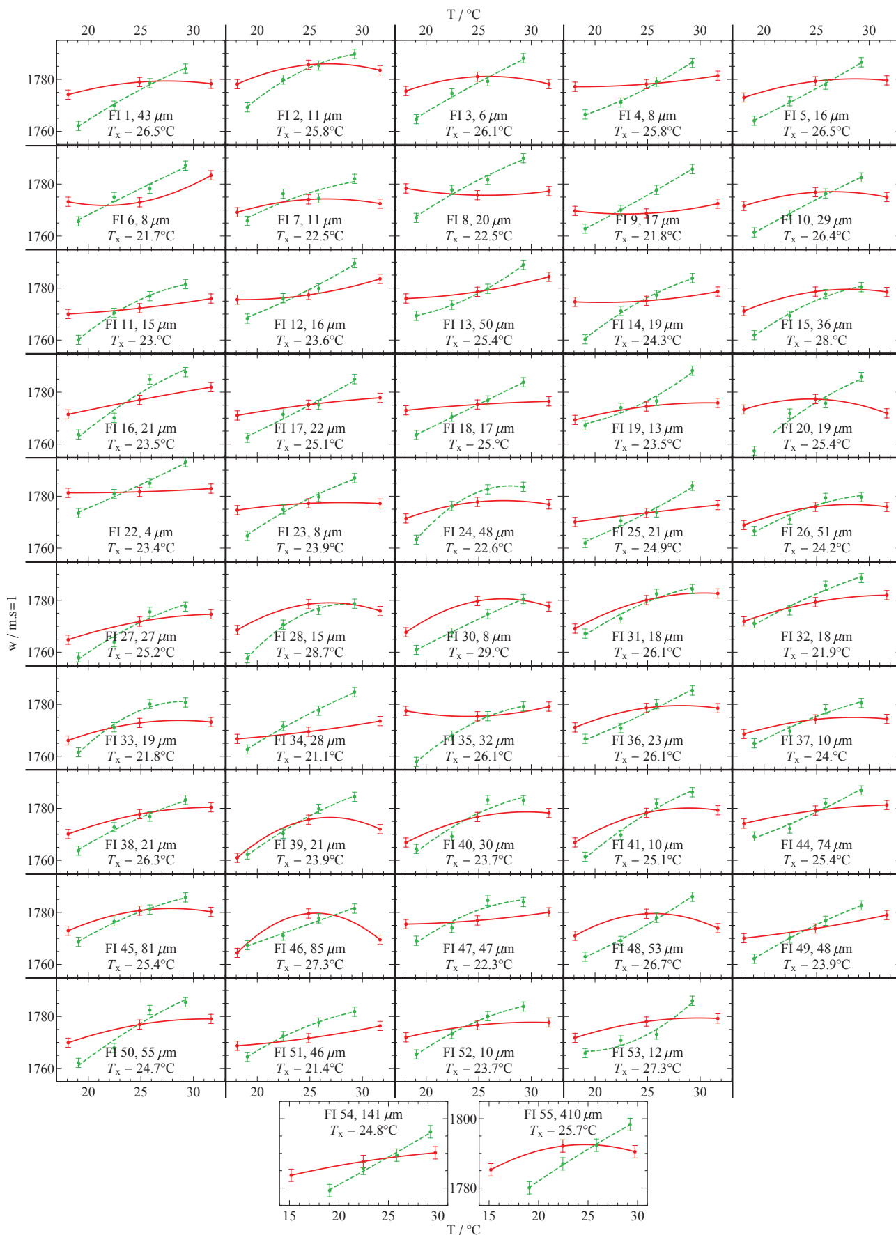
Figure 3.A.1: Individual LVE (red disks) and isochore (green disks) w measurements in SyntHal24.619 FIs. Parabolas are fitted to the LVE data points (red solid curve) and the iso- T_h data points (green dashed curve). T_x is the temperature of intersection.
