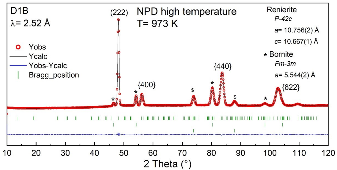
Figure 2.21. Le Bail refinement of the NPD pattern at 973 K. The main phase is refined with a P\bar{4}2c ( a = 10.756(2) Å, c = 10.667(1) Å) space group and a Fm\bar{3}m ( a = 5.544(2) Å) space group for bornite (identified by an asterisk). A dollar sign marks the thermocouple contribution.
