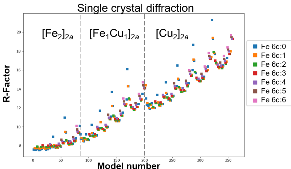
Figure 4.8. R-Factors obtained from the refinement of the 360 structural models with variable Fe content on the 6d site on single crystal data ( \lambda_{M0} ).
