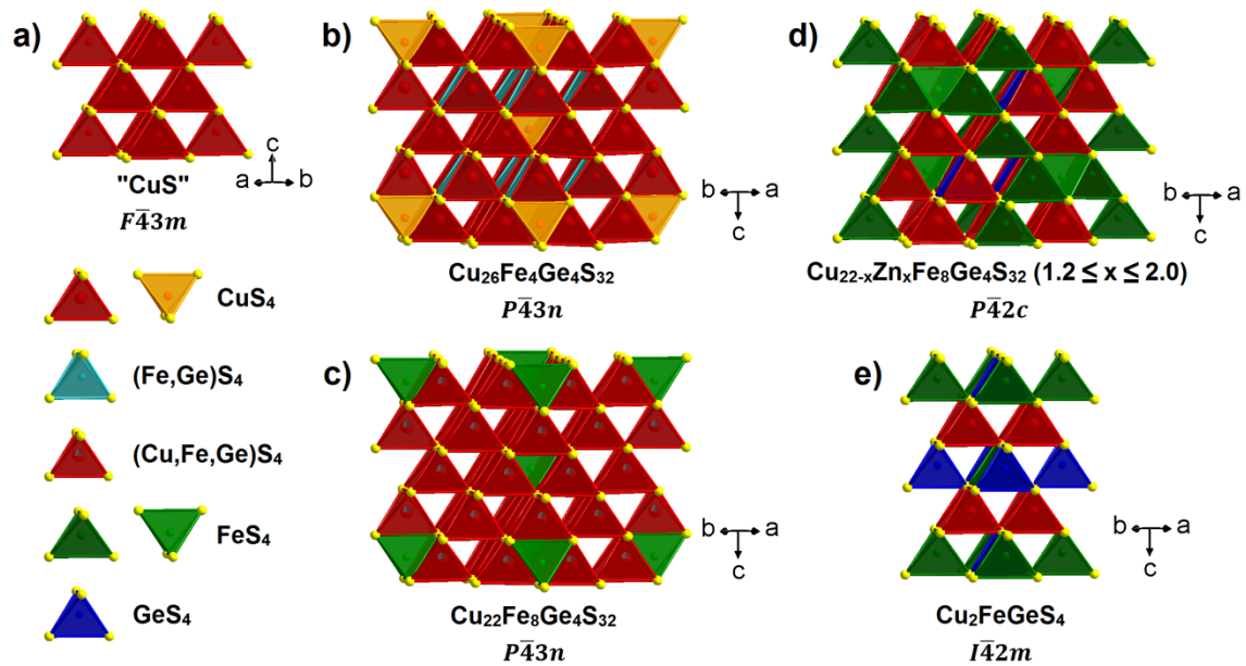
Figure 3.1. Crystal structure representations highlighting the semi-ordered cation distribution of a) sphalerite "CuS", b) mineral germanite Cu_{26}Fe_4Ge_4S_{32} , c) synthetic germanite Cu_{22}Fe_8Ge_4S_{32} , d) renierite Cu_{22-x}Zn_xFe_8Ge_4S_{32} ( 1.2 \leq x \leq 2.0 ) and e) briartite Cu_2FeGeS_4 .
