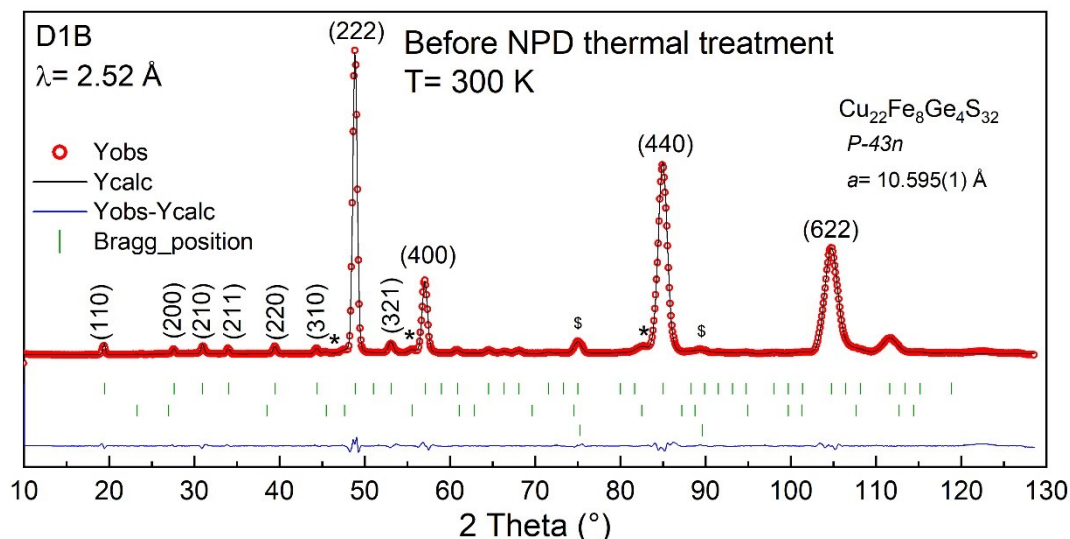
Figure 2.14. Le Bail refinement of germanite \text{Cu}_{22}\text{Fe}_8\text{Ge}_4\text{S}_{32} ( P\bar{4}3n , a = 10.595(1) Å) measured by NPD at RT. The bornite ( Fm\bar{3}m , a = 10.852(7) Å) contributions are pinpointed by an asterisk and that of the thermocouple by a dollar sign.
