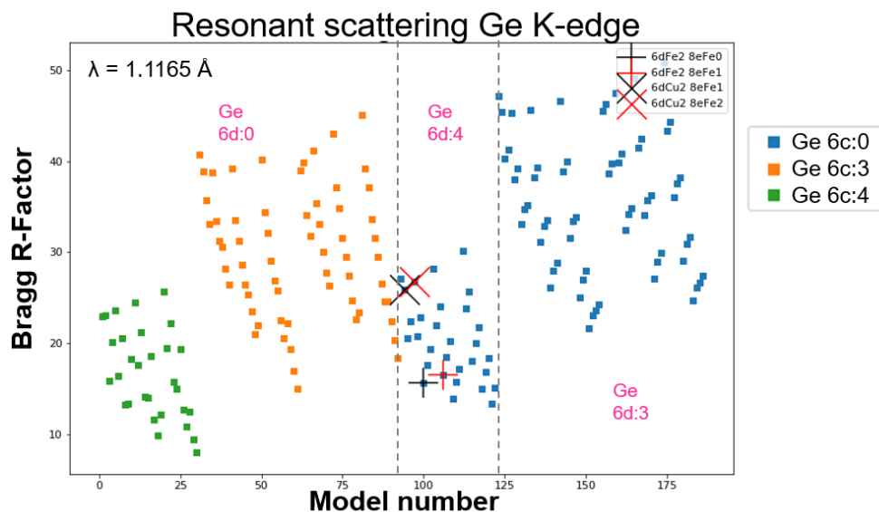
Figure 4.14. Bragg R -Factors obtained from the Rietveld refinement of the 186 structural models at Ge K-edge. The plot is divided in 3 zones corresponding to the Ge occupation of the 6d site. A color identifies each 6c occupation.
