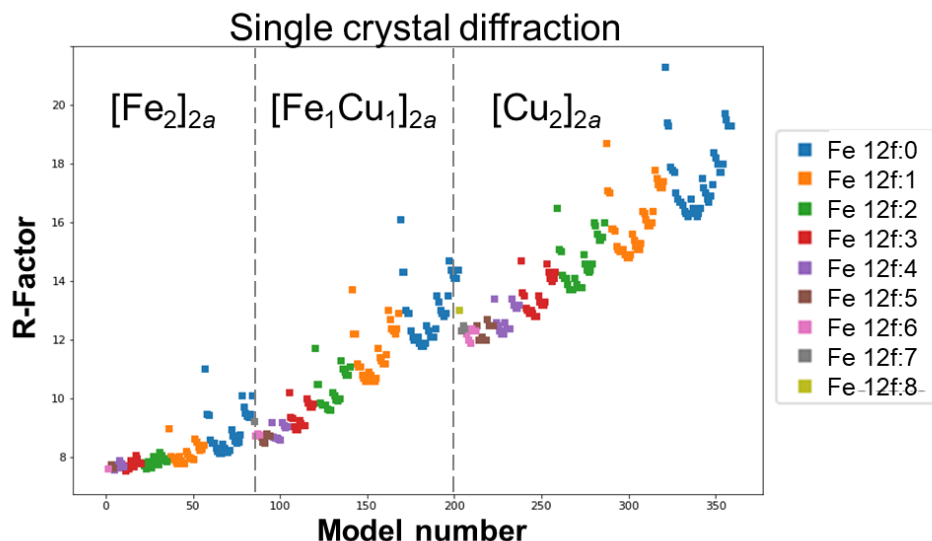
Figure 4.7. R-Factors obtained from the refinement of the 360 structural models with variable Fe content on the 12f site on single crystal data ( \lambda_{M0} ).
