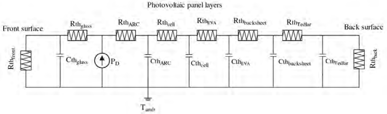
Fig. 29 Photovoltaic thermal resistance network.
