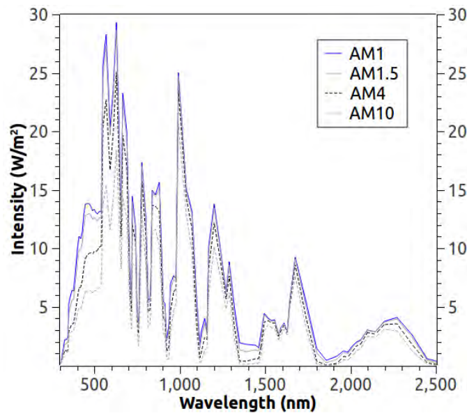
Fig. 66 Solar spectral irradiance for different values of AM coefficient (for Strasbourg, France, on May 15 th , 2015).
