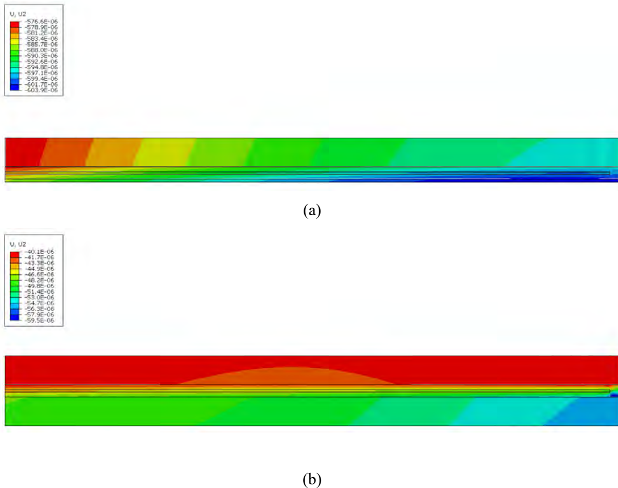
Fig. 98 Vertical displacement at nodes (or deflection, plotted in [m]) predicted under NOCT for VSMS275 (a) and Panasonic225 (b) PV panels.
