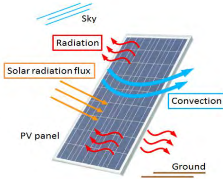
Fig. 27 Representation of the heat exchange with the outside.
