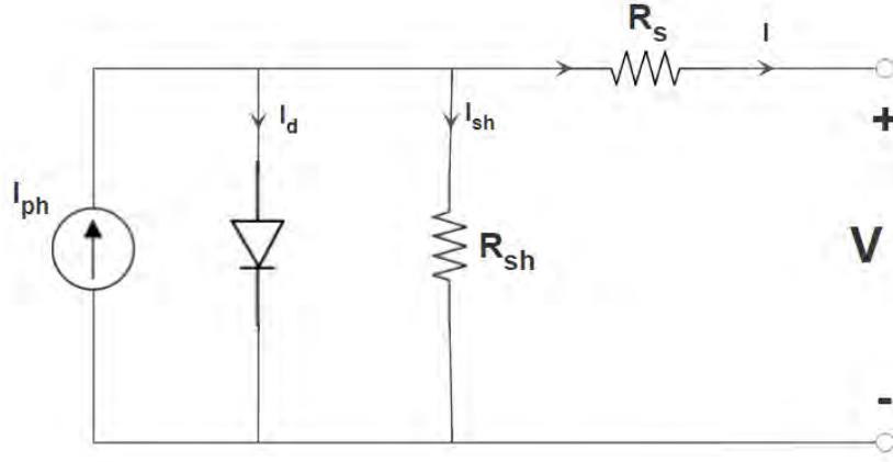
Fig. 33 One diode model equivalent electrical circuit.
