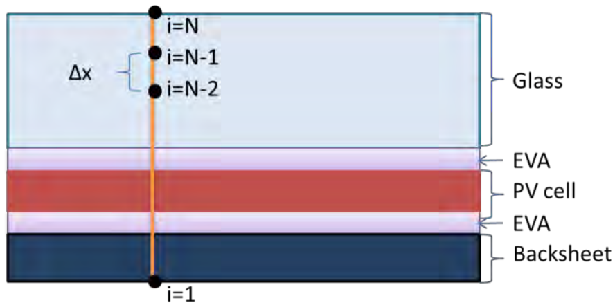
Fig. 30 PV panel layers in 1D approach.
