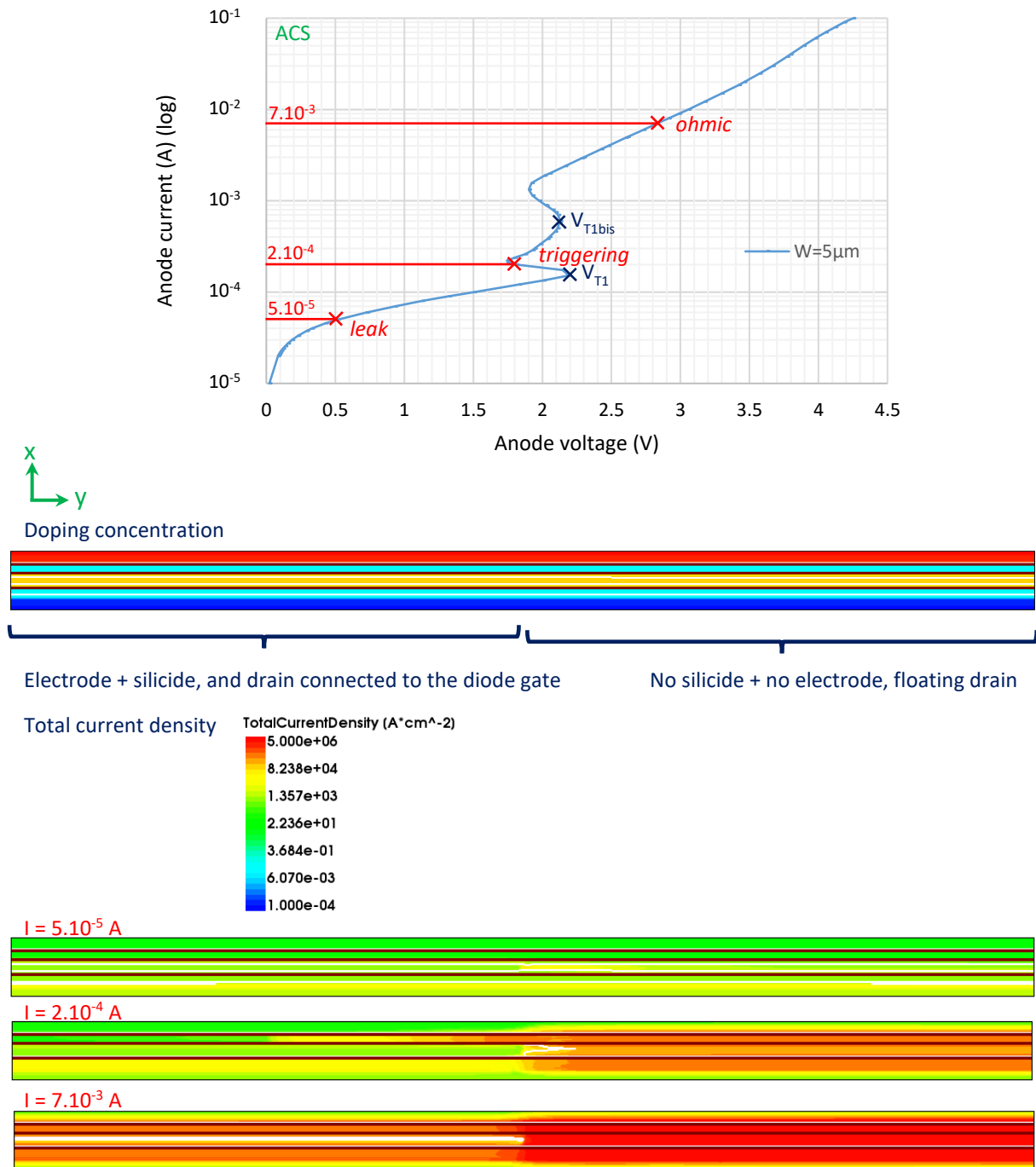
Figure 96: Top: I-V TCAD ACS simulation of a N-LDD GDNMOS with the drain (with a cover of silicide of 5 \mu m out of 10 \mu m of finger) connected to the diode gate and a grounded NMOS gate. Bottom: extracted top views from the structure.
