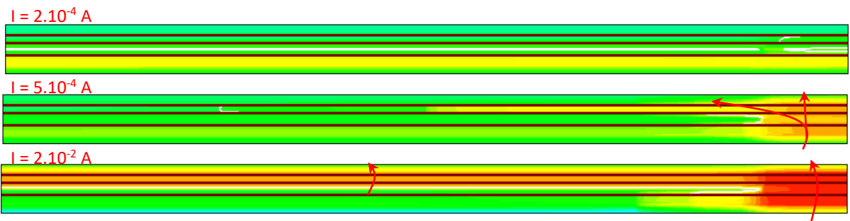
Figure 103: Top: I-V TCAD ACS simulation of a N-LDD GDNMOS with grounded gates and the drain connected to the anode on a silicided part of the width of the drain. W_{\text{silicide}} = 9 \mu\text{m} . The contribution of the anode and the drain are detailed in the total current flowing through the device. Bottom: extracted views from the structure.
