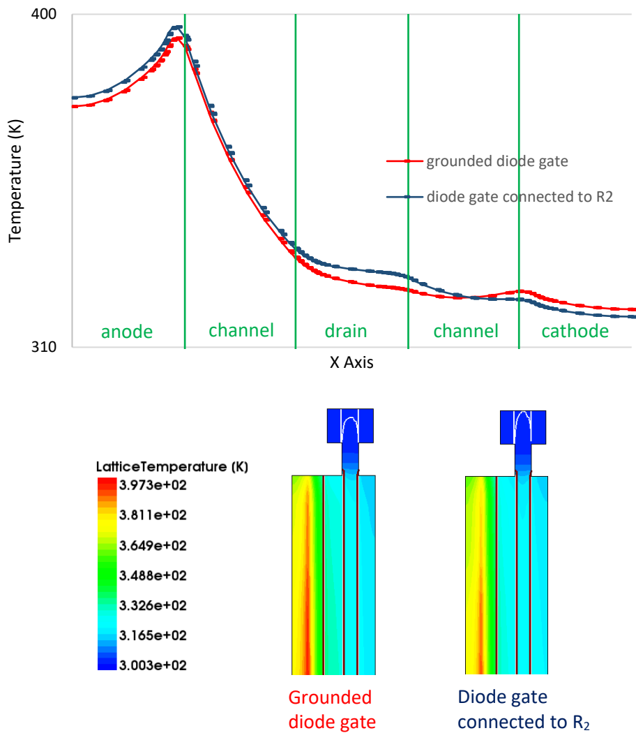
Figure 80: Temperature extraction during ACS stress in thermodynamic simulation for an anode negative current of I = 3 \cdot 10^{-3} \text{ A} (see Figure 79) in a GDBIMOS with both gates plugged to the resistor R_2 , and in a GDBIMOS with only the BIMOS gate plugged to the resistor R_2 and the diode gate grounded.
