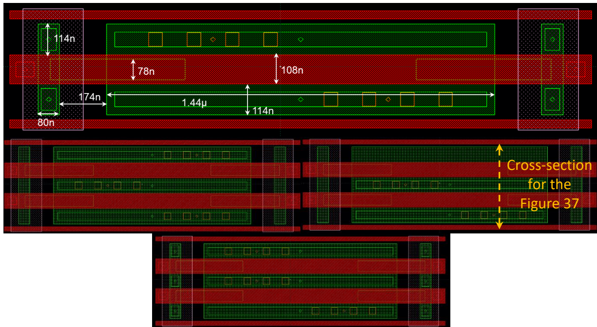
Figure 35: Layouts. Top: BIMOS_1finger and its dimensions; Middle left: BIMOS_2fingers; Middle right: BIMOS_capabooft_float; Bottom: BIMOS_capabooft. The orange squares show where the contacts are situated; there is one metal line for connecting the drain (left of each device) and one for the source (right of each device) but it is not displayed.
