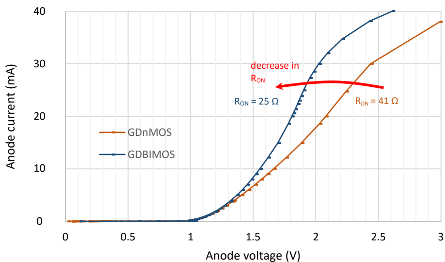
Figure 74: Electro-thermal ACS I-V TCAD characteristics of a GDNMOS and a GDBIMOS. Both devices have their gates connected to the resistor R_2 and N-LDD doping.
