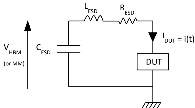
Figure 8: HBM and MM models and associated parameters.
