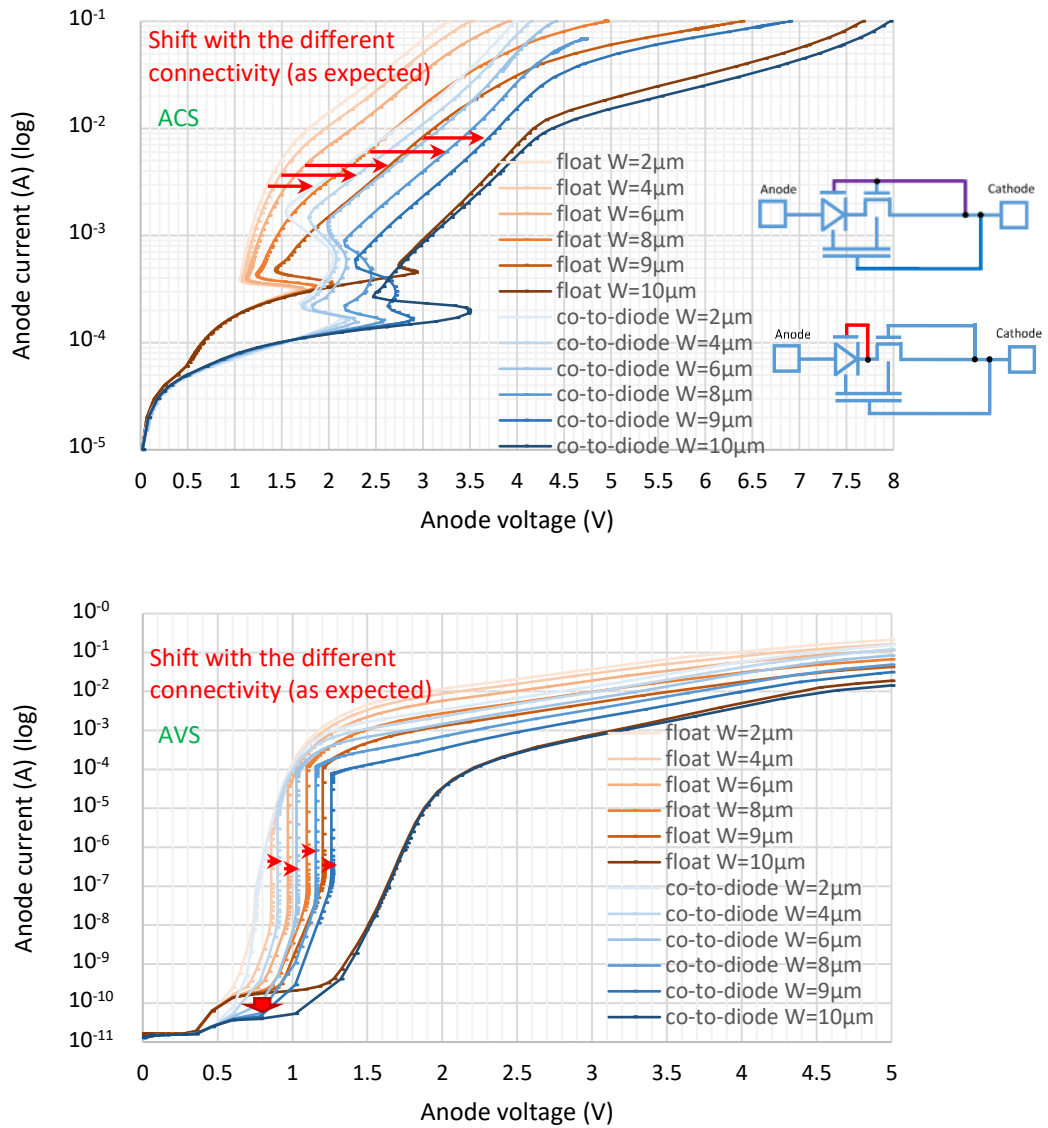
Figure 94: I-V TCAD simulation of a N-LDD GDNMOS with a grounded NMOS gate, for different silicide covers of the drain. “float” (the drain is left floating and the diode gate is grounded) is compared to “co-to-diode” (the drain is connected to the diode gate). Top: ACS. Bottom: AVS.
