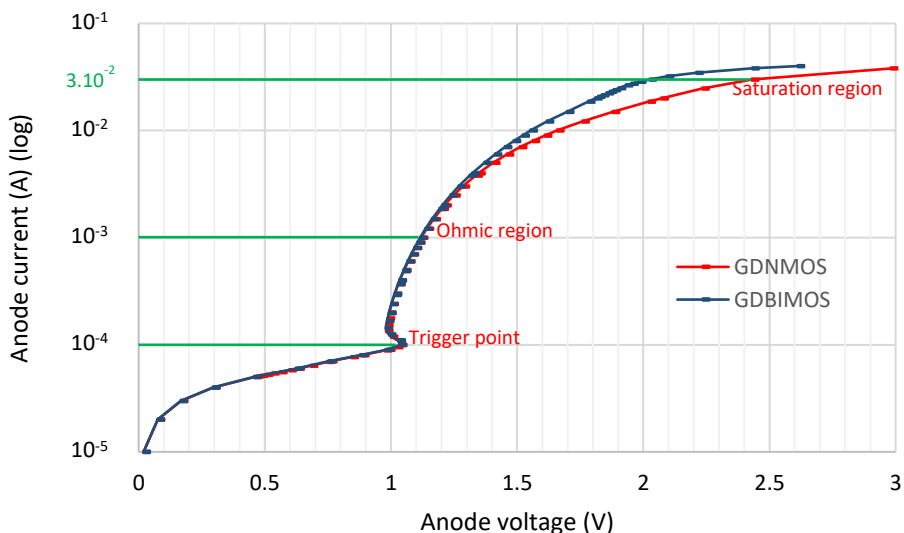
Figure 76: Electro-thermal ACS I-V TCAD simulation of a GDNMOS and a GDBIMOS with both gates connected to the resistor R_2 . Those are the same curves than the ones in the Figure 74, except that the current is displayed with a logarithmic scale.
