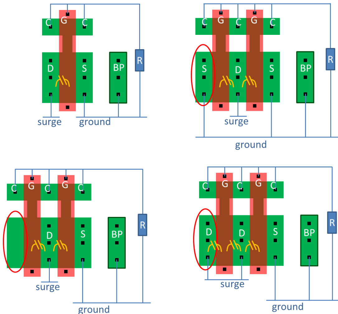
Figure 34: Top views of BIMOS and their connectivity. Top left: BIMOS_1finger; Top right: BIMOS_2fingers; Bottom left: BIMOS_capaboost_float; Bottom right: BIMOS_capaboost. The colors correspond to cadence virtuoso layers, like for Figure 35 (active in green, gate stack in red). The parasitic capacitances are displayed in yellow. Note the connectivity of the additional finger (encircled in red).
