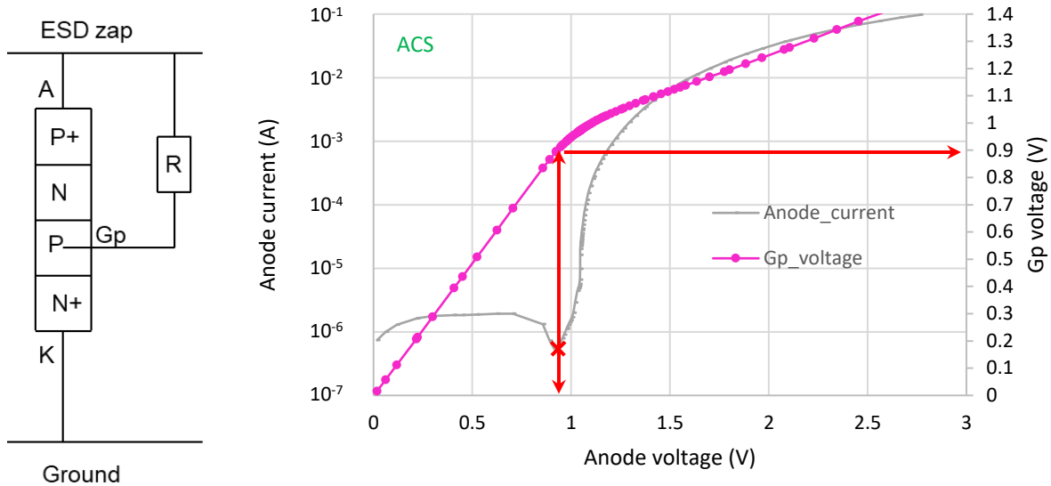
Figure 149: Left: schematic of the studied SCR; a resistor has been plugged between Gp and the anode (subject to the surge). Right: TCAD ACS simulation of the SCR shown left. The triggering of the SCR occurs when the body contact is around 0.89 V.
