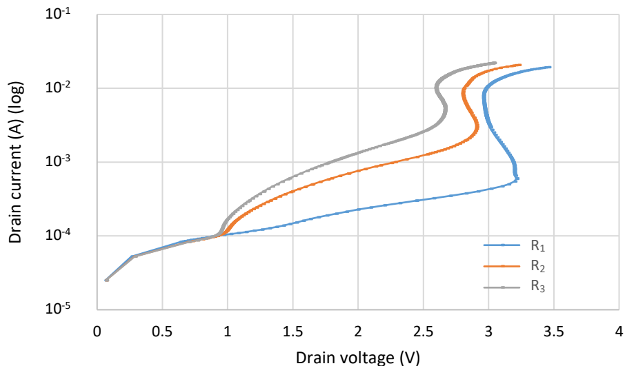
Figure 41: Electro-thermal ACS TCAD simulation. BIMOS_capaboost, with different values of external resistor ( R_1 < R_2 < R_3 ).
