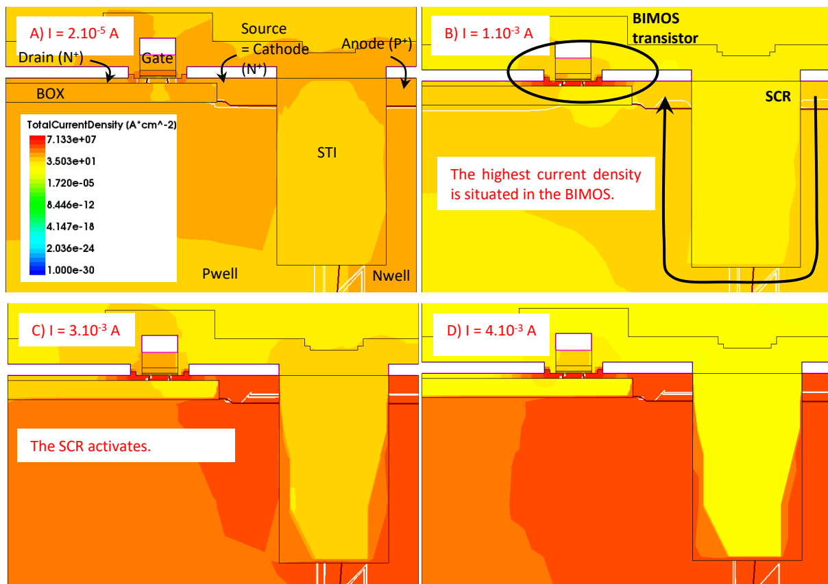
Figure 148: Extracted current density in cross section C2 (see Figure 143) of the merged device from the curve in Figure 147 (points A, B, C and D).
