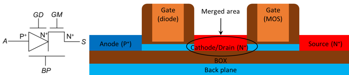
Figure 29: Schematic (left) and cross-section (right) of a GDNMOS structure.
