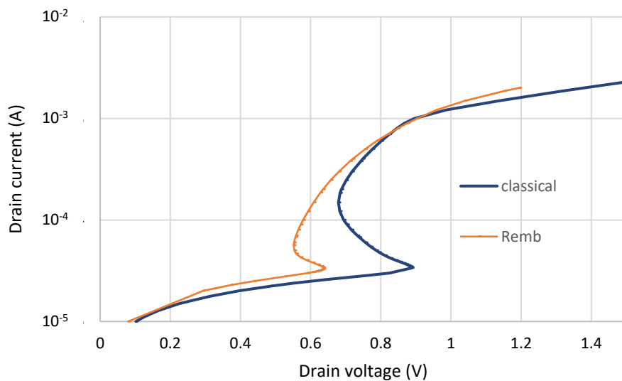
Figure 163: TCAD reverse ACS simulations of a 48 nm gate length and 2 \mu\text{m} gate width BIMOS. “classical” (without BOX opening, and with an external resistor of R_3 plugged between the gate + body contacts and the “ground”) in the legend is opposed to “Remb” (with openings in the two body contact regions, and the first body contact is plugged to the gate while the second one is grounded).
