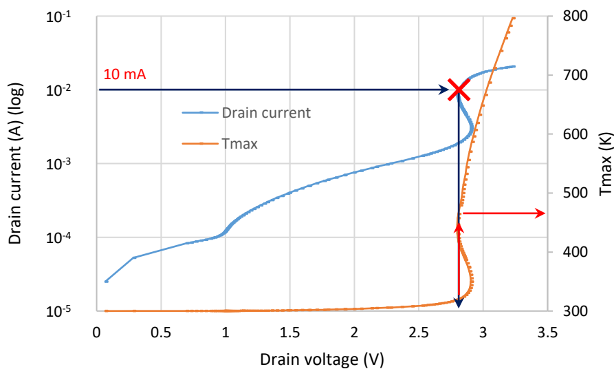
Figure 36: Electro-thermal ACS TCAD simulation. Thermal response of the BIMOS_capaboost. Figure 37 is obtained by plotting the device when the current is 10 mA, which corresponds to the emphasized point on this graph.
