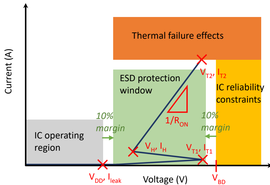
Figure 14: ESD design window.
