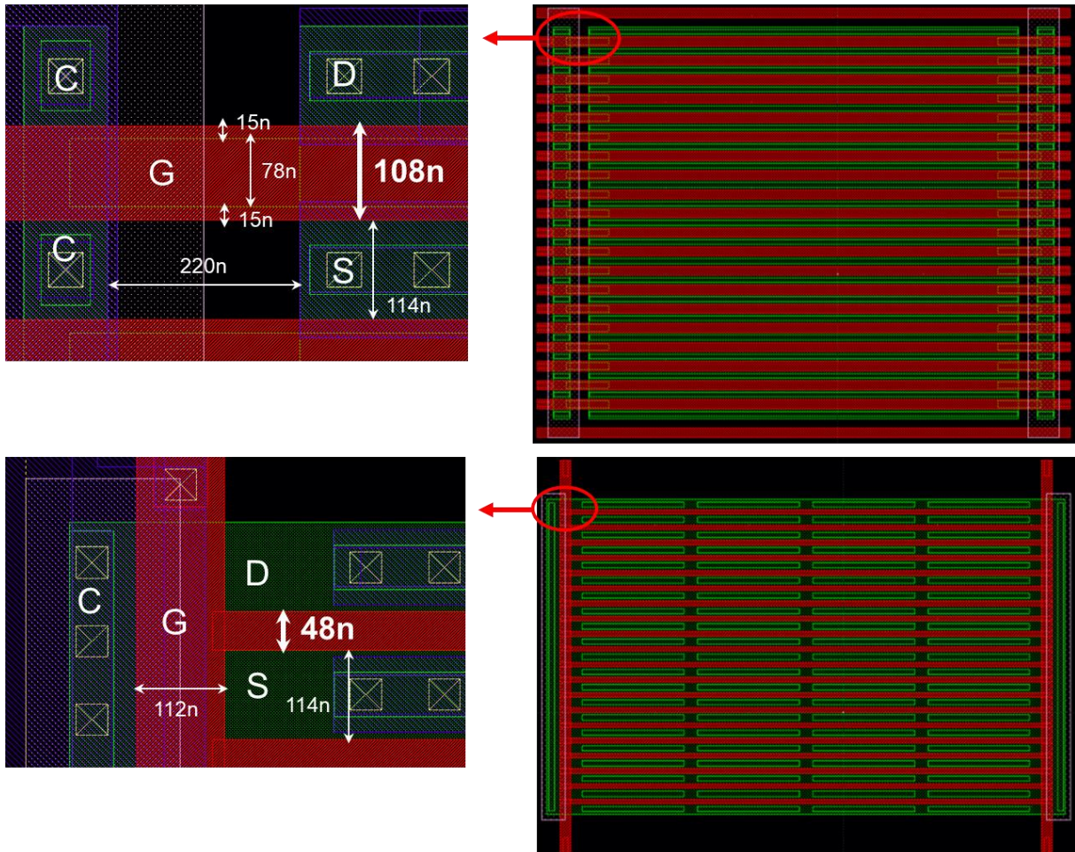
Figure 111: Top: Classical BIMOS. Bottom: T-gate BIMOS. Right: multi-finger layout (20 fingers of 5 μm). Left: zoom and dimensions. Note that the classical BIMOS is very constrained in terms of dimensions because of the bridge of active (to link the body contacts and the source and drain) that must be covered by the gate. D, S, C and G respectively stand for Drain, Source, Body Contact and Gate.
