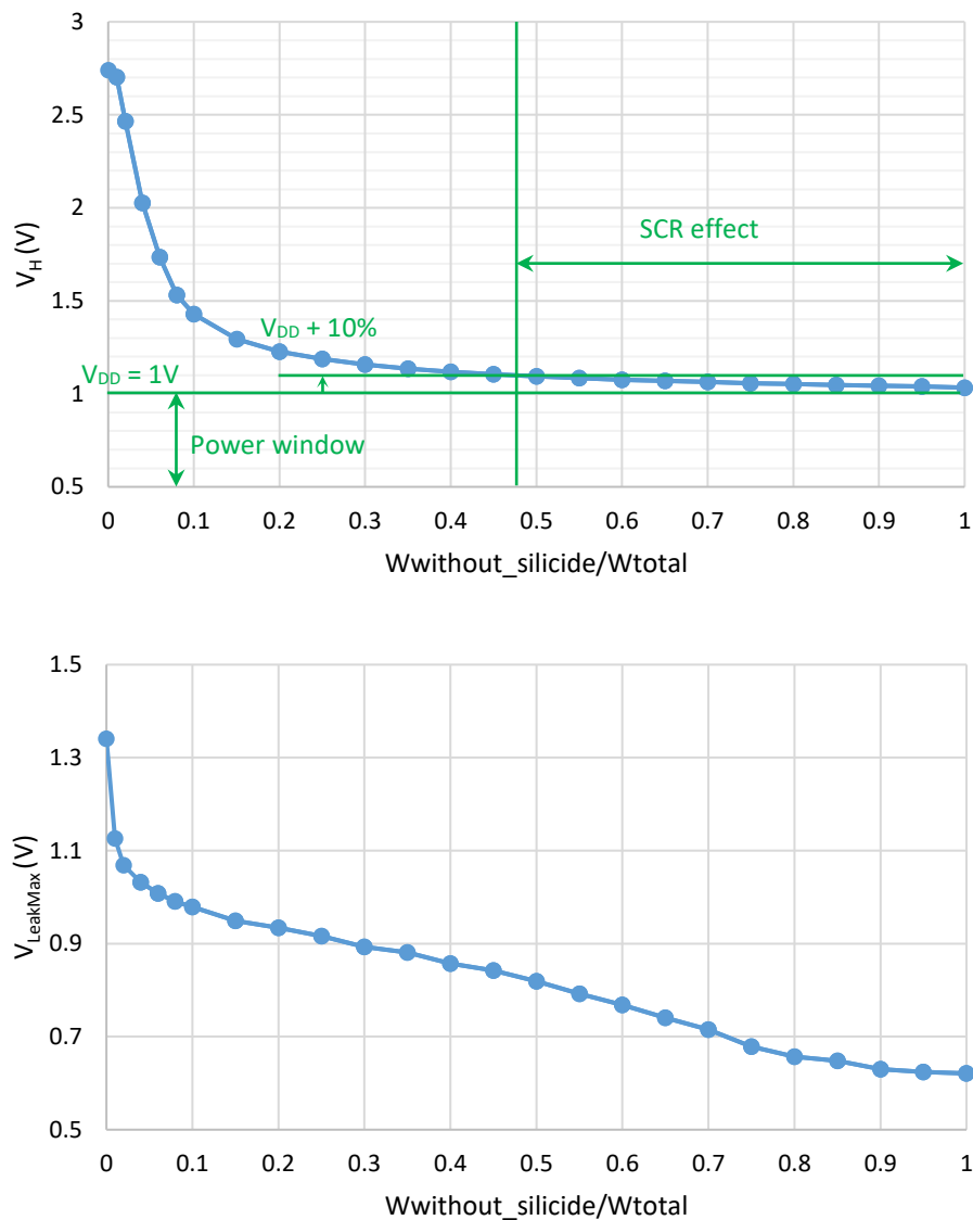
Figure 91: Holding voltage V_H (extracted from the ACS curve) and maximum voltage allowed as a V_{DD} in terms of leakage current for the protection V_{\text{LeakMax}} (it is the voltage at 1 nA on the AVS curve) versus the proportion of width without silicide and the total width of the finger. Note that W_{\text{without\_silicide}} = W_{\text{total}} - W_{\text{silicide}} . When there is few silicide, the SCR effect is present in the device and the holding voltage V_H is close to V_{DD} = 1V ; as a result, the device is immune to latch up if there is a sufficient width of silicide on the drain.
