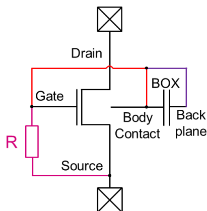
Figure 25: Schematic of a thin-film BIMOS structure.
