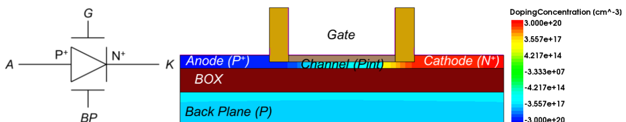
Figure 22: Schematic of a diode (left), and TCAD view of a thin-film gated diode.
