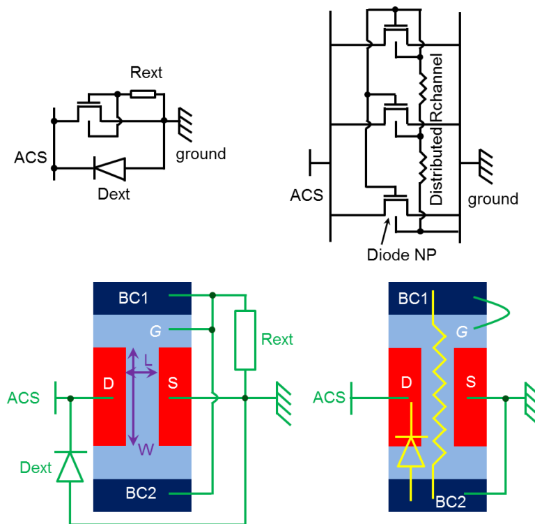
Figure 155: Top: schematics. Bottom: Top view of the T-gate BIMOS topology with two body contacts, with the external connectivity in green and the internal elements in yellow. Left: External resistor (classical circuit). Right: Embedded resistor (new circuit).
