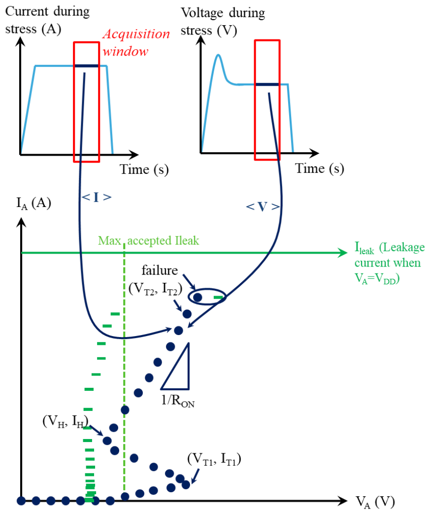
Figure 20: Top: Principle of TLP measurement. Square pulses are sent, then the voltage and current are measured to draw the I-V characteristic. Bottom: Typical I-V curve of an ESD protection device, with its leakage (green scale).
