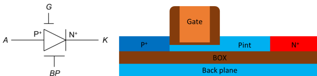
Figure 28: Schematic (left) and cross-section (right) of a Z 2 -FET structure.
