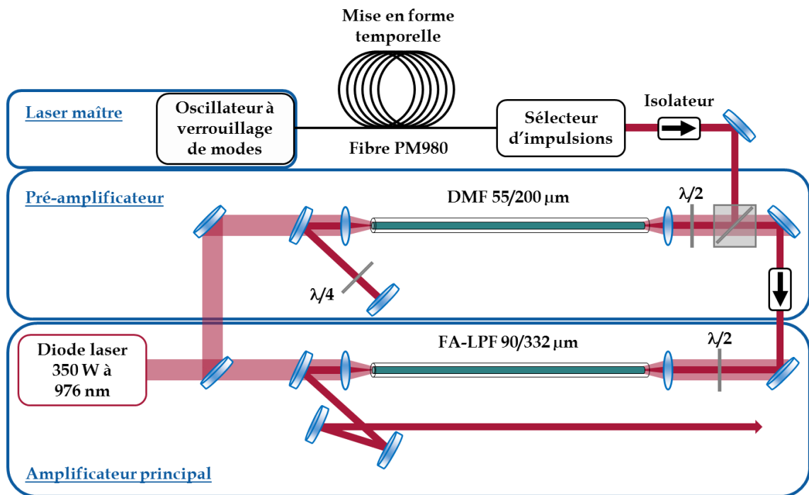
Figure IV-8 – Architecture laser industrielle MOPA picoseconde à 1030 \text{ nm} .
