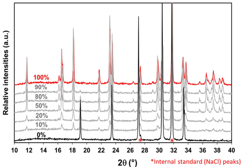
Figure III-6 : XRPD patterns of samples recrystallized in water and analyzed with NaCl as internal standard: 100% \text{NaClO}_3 (0% of \text{Na}_2\text{S}_2\text{O}_6 \cdot 2\text{H}_2\text{O} ) in black, 100% \text{Na}_2\text{S}_2\text{O}_6 \cdot 2\text{H}_2\text{O} in red and different compositions in grey. Percentage of \text{Na}_2\text{S}_2\text{O}_6 are indicated on respective XRPD patterns. Red stars indicate aligned peaks of the internal standard (NaCl).
