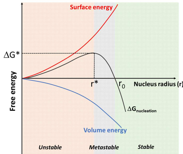
Figure I-8: Schematic representation of the evolution of the nucleation free enthalpy \Delta G_{\text{nucleation}} versus the nucleus radius ( r ) (black curve). The negative contribution linked to the volume energy and the positive contribution due to the surface energy are represented by blue and red curves respectively. Unstable, metastable and stable domains are colored in orange, grey and green respectively.
