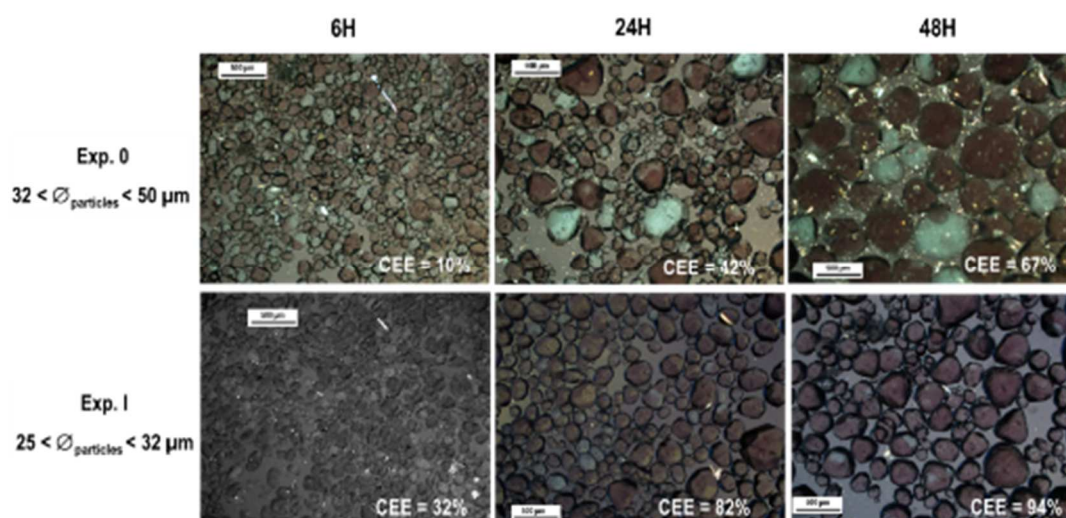
Figure IV-8 : POM Pictures of \text{NaClO}_3 crystals after 6, 24 and 48 hours in the deracemization experiments in the CT reactor for initial crystal size between 32 and 50 \mu\text{m} (top), and for initial crystal size between 25 and 32 (bottom). The inlays indicate the %CEE.
