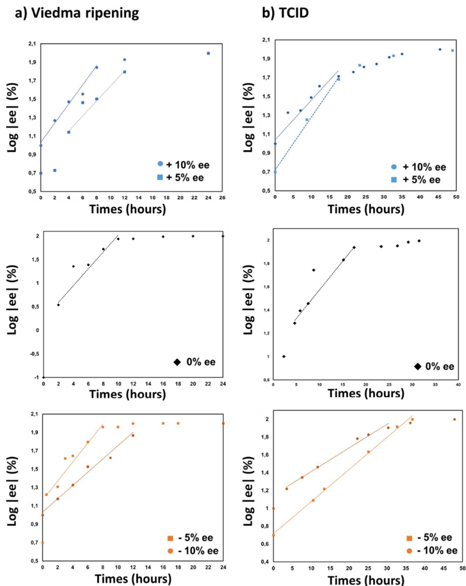
Figure II: Evolution of the \text{log } |ee| (%) as a function of the time of a) VR experiments and b) TCID experiments. The line is the linear regression, detailed in table I. Inlay indicates the starting ee_{\text{crystal}} .
