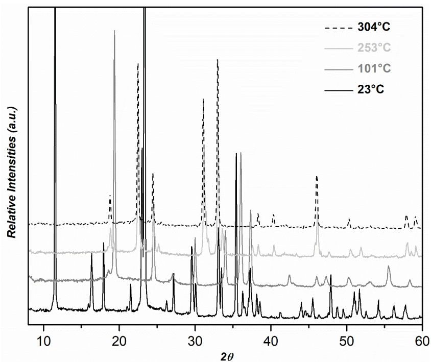
Figure II-4: TR XRPD performed on synthesized \text{Na}_2\text{S}_2\text{O}_6 \cdot 2\text{H}_2\text{O} at: room temperature (black line), 101 °C (dark grey line), 253 °C (light grey line), and 304 °C (black dashed line).
