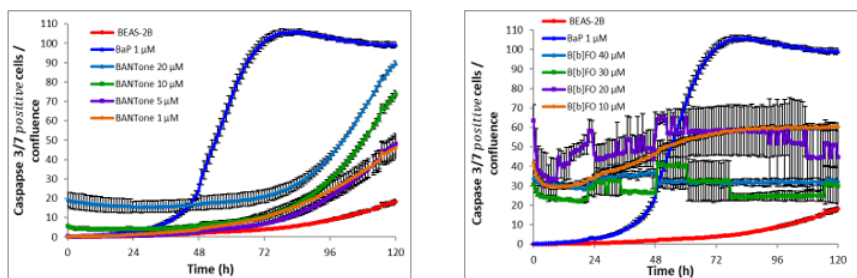
Figure 2. Investigation of the mechanism of cellular death on BEAS-2B cells exposed to oxy-PAHs. A. Cells observed I microscopy by IncuCyte® S3 acquiring images (objective x 10) at 24 hours of exposure. B. Analysis of the cell cycle at 24 hours of exposure. C. CellTox™ Green assay after exposure during 24 hours. The reagent was added after the exposure. The upper plot represents time after treatment as a function of green fluorescence. For the lower plot, time after treatment is represented as a function of confluence. D. Kinetic quantification of caspase-3/7 mediated apoptosis after exposure during 24 hours. The reagent was added after 24 hours of exposure.
