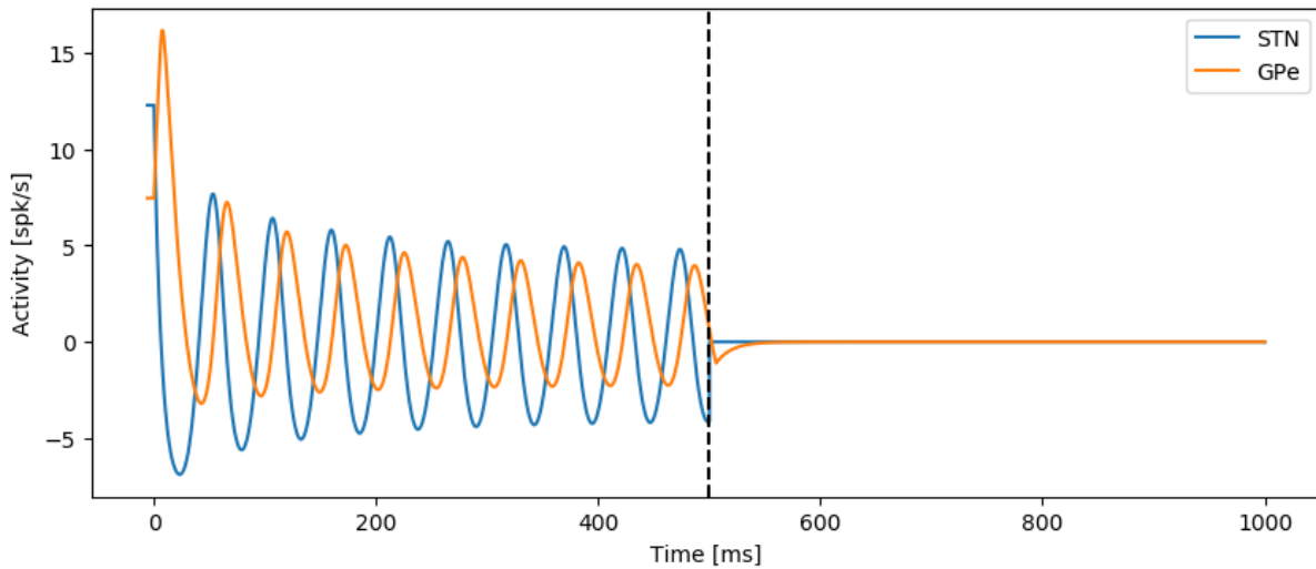
Fig. 2.2: Stability of the firing rate model (2.7) under proportional feedback with \theta estimated from Proposition 10. Proportional stimulation with \theta = \hat{\theta}^* is applied from t = 500 ms. Since \hat{\theta}^* is a rough estimate, way higher than necessary, proportional feedback disrupts the oscillations almost instantaneously.
