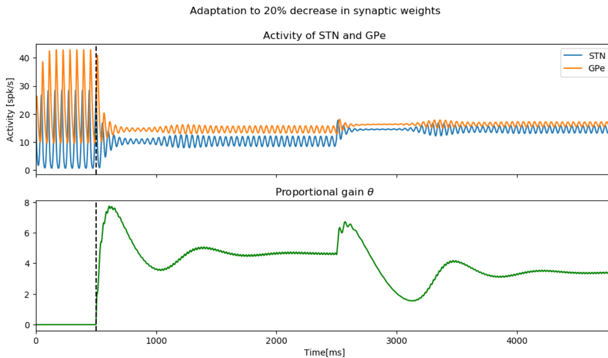
Fig. 4.7: Adaptation to decrease of synaptic weights
