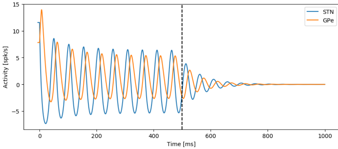
Fig. 2.1: Stability of the firing rate model (2.7) under proportional feedback. Proportional stimulation with \theta = 5 is applied from t = 500 ms. Under proportional stimulation the feedback system is exponentially stable, so it converges to the origin.
