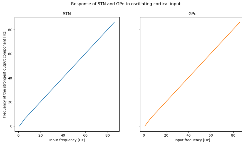
Fig. 5.7: Under condition (5.7), the frequency of oscillations of (5.1) is identical to frequency of the sinusoidal input applied to STN. This is a consequence of (5.1) being incrementally stable.
