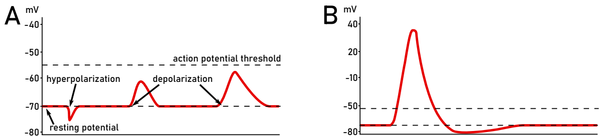
Fig. 1.2: Illustration of a neuron response to stimulation. A : Isolated subthreshold hyperpolarization and depolarization events do not induce action potentials and the neuron reverts to the resting potential. B : Superthreshold stimuli cause the neuron to generate an action potential.
