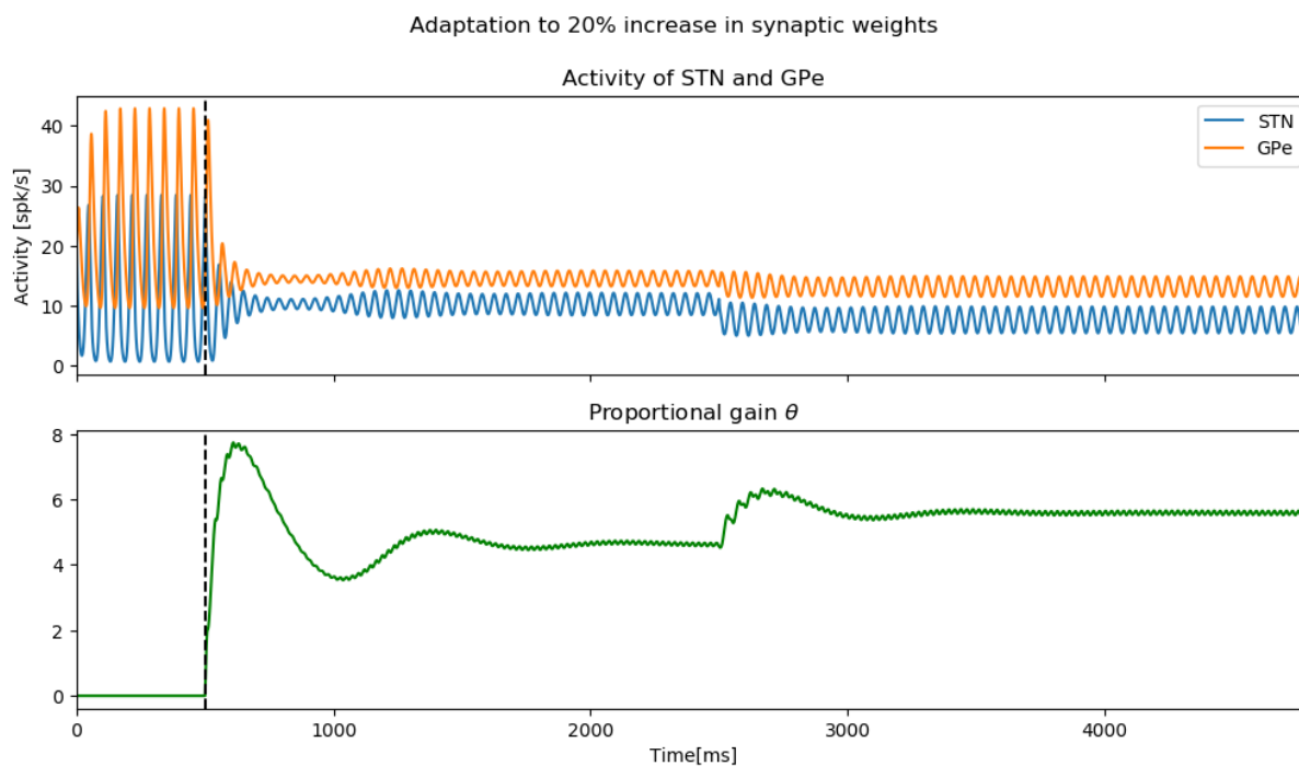
Fig. 4.8: Adaptation to increase of synaptic weights
