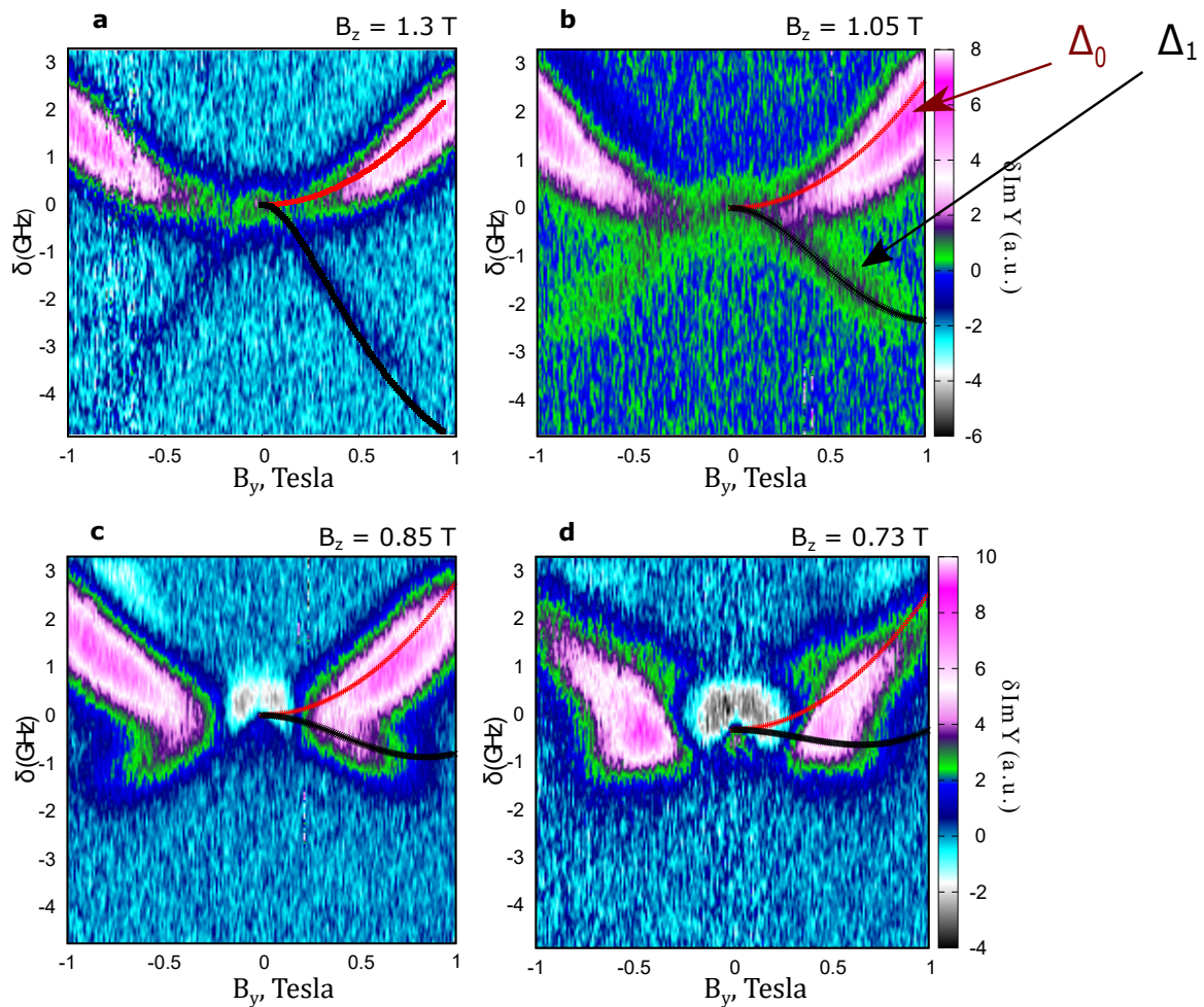
Figure 11.6: QED Hamiltonian calculations results overlaid on the experimental maps from figure 11.4. Red and black curves give the QED Hamiltonian predictions for the \Delta_0 and \Delta_1 transitions drawn in figure 11.5 between states |n, m\rangle .
