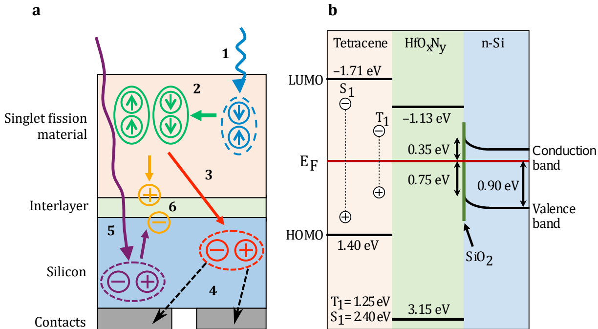
Figure 2.7: Markus Einzinger et al. 's singlet fission sensitized solar cell scheme. a , (1) Light absorption in tetracene, (2) singlet fission, (3) energy transfer to silicon, (4) charge separation, (5) light absorption in silicon, (6) electric field passivation. b , Energy transferring scheme. Illustration is adapted from Ref. [61].
