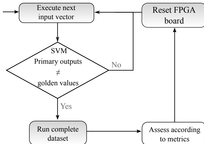
Fig. 4.16: Method used on the radiation test
