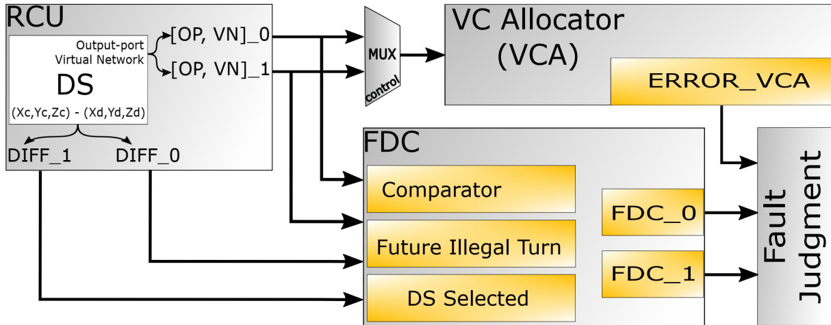
Fig. 2.7: Fault detection Circuit - FDC.
