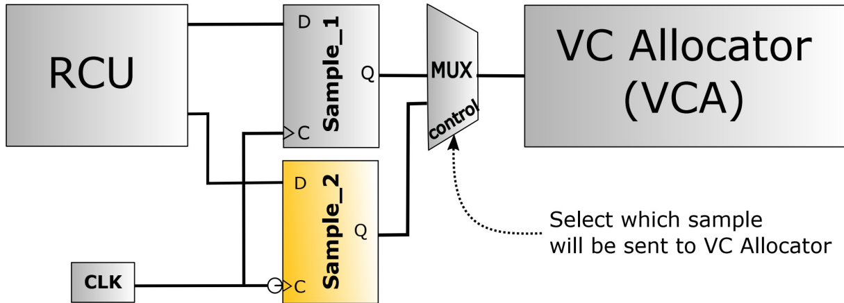
Fig. 2.6: A Double-Sampling implementation.
