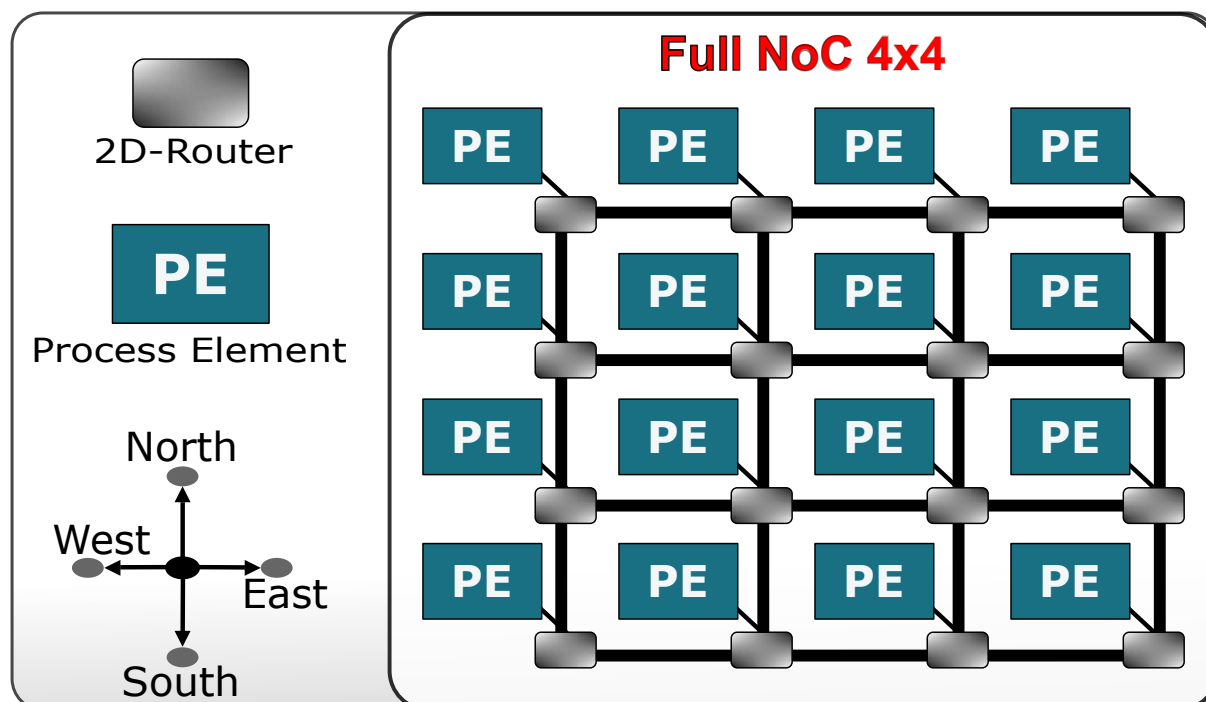
Fig. 5.1: A 4x4 two-dimensional Networks-on-Chip.
