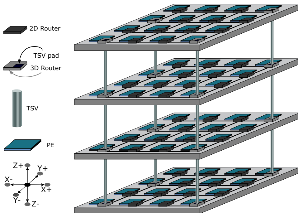
Fig. 3.1: 3D-NoC architecture vertically and partially connected
