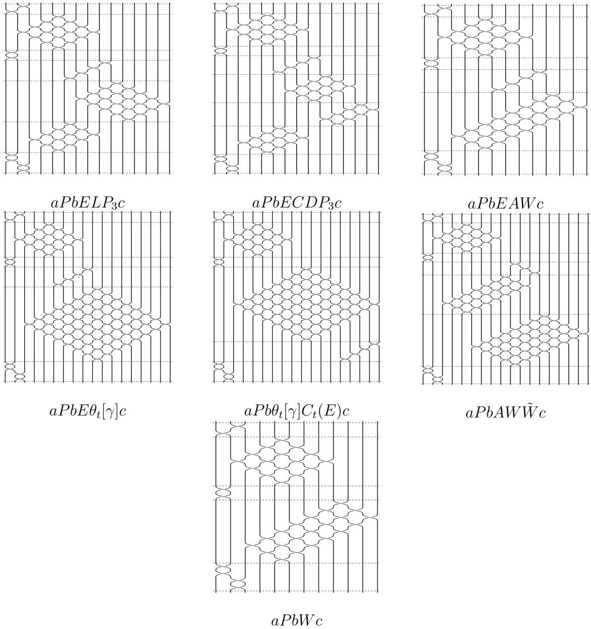
Figure 2.8: The equality a\theta_{\nu}[\beta]b\theta_k[\gamma]c = aPbWc .
