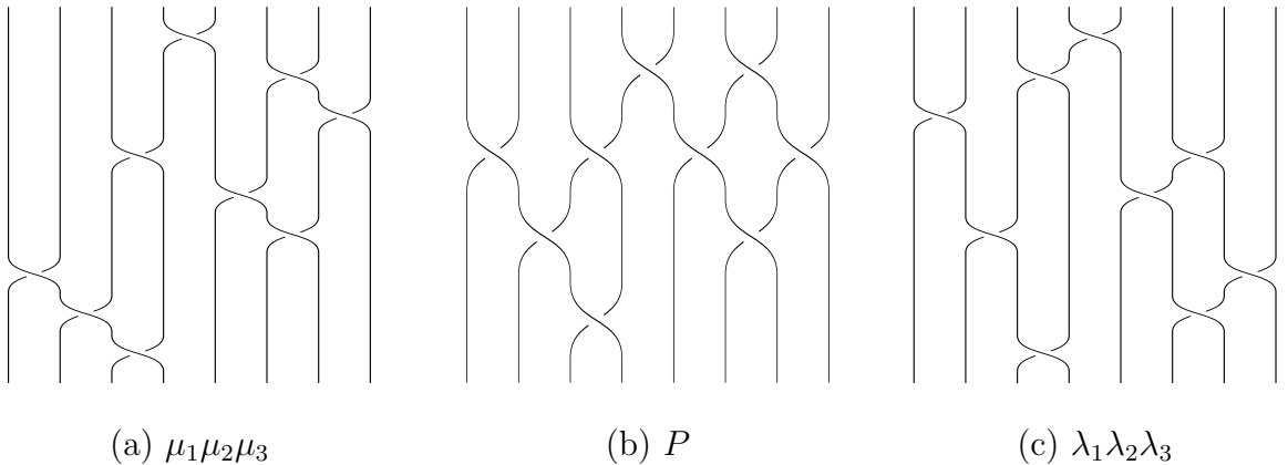
Figure 2.5: The equality \mu_1 \mu_2 \mu_3 = P = \lambda_1 \lambda_2 \lambda_3 .
