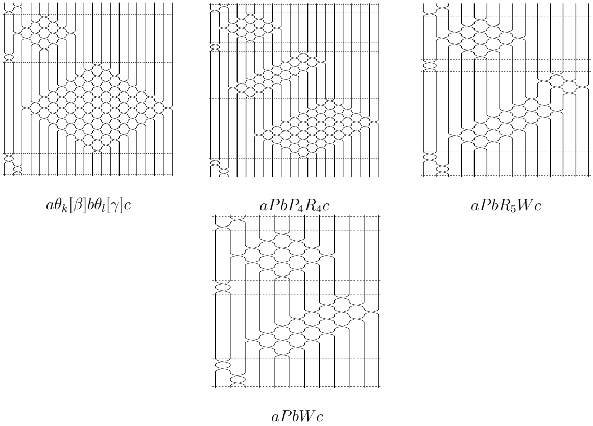
Figure 2.7: The equality a\theta_k[\beta]b\theta_l[\gamma]c = aPbWc .
