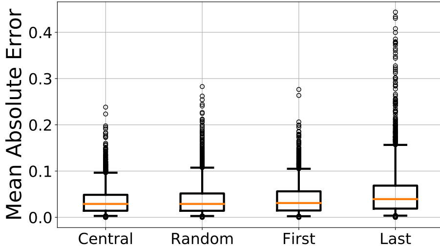
Figure 6.5: Missing value imputation for 4 different scenarios : imputation of the central, a random, the first or the last value.
