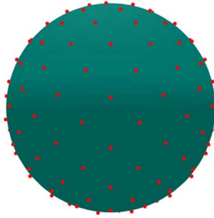
Figure 4.8 – Uniform sampling of the sphere.
