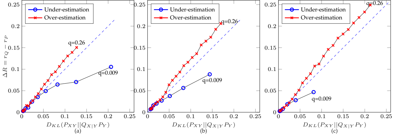
Figure 5.4 – Excess rate under mismatched decoding metric Q_{XY}(x, y) = Q_{X|Y}(x|y)P_Y(y) as a function of D_{KL}(P_{XY} || Q_{X|Y} P_Y) for the non-symmetric channel from Y to X . Each point shows the excess rate for a specific Q_{X|Y}(0|1) = Q_{X|Y}(1|0) = q . The dashed line is the identity line D_{KL}(P_{XY_i} || Q_{X|Y_i} P_{Y_i}) . (a) P_Y(0) = 0.1 . (b) P_Y(0) = P_Y(1) = 0.5 . (c) P_Y(0) = 0.9 .
