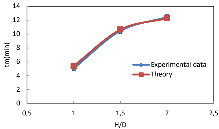
Figure 2.20: Theoretical and experimental mean residence time measured in different operating conditions (H/D=1, 1.5 and 2).
