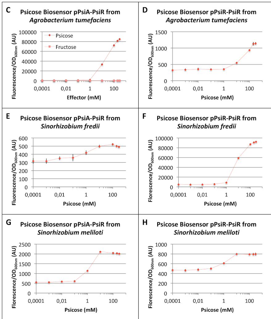
Figure 5.1. Design and characterisation of six psicose biosensors. (A) Schematic representation of the Universal Biosensing Chassis (UBC) used as a platform to build the psicose biosensors (B). (C-H) In vivo characterisation of mCherry expression by E. coli cells harbouring (C) the psicose biosensor based on pPsiA promoter from Agrobacterium tumefaciens and the PsiR transcription factor from Agrobacterium tumefaciens (BBa_K2448025), (D) the psicose biosensor based on pPsiR promoter from Agrobacterium tumefaciens and the PsiR transcription factor from Agrobacterium tumefaciens (BBa_K2448026), (E) the psicose biosensor based on pPsiA promoter from Sinorhizobium fredii and the
