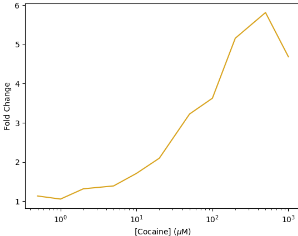
Supplementary Figure S8.14. Detection of cocaine spiked into clinical urine samples with sfGFP output module. A standard gradient of cocaine hydrochloride was added with 2 μL of a human urine sample to 20 μL cell-free reactions containing our optimized cocaine biosensor with 0.8 U/μL of a murine RNase inhibitor and incubated at 30°C for 12 hours. Fold change was calculated relative to the 0 μM cocaine inducer. Data are from a single pilot experiment.
