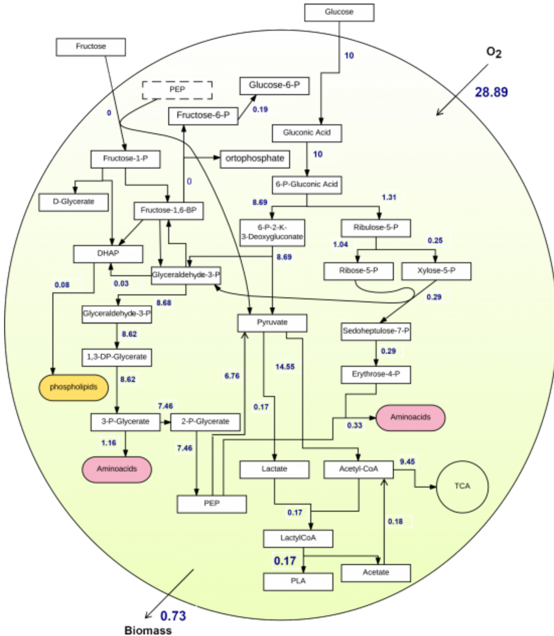
Figure 4.4. Schematic representation of the central metabolism with PLA pathway, using glucose as substrate and considering PLA as biomass precursor. In this flux distribution, glucose is the carbon source and PLA has been set as a precursor of biomass.
