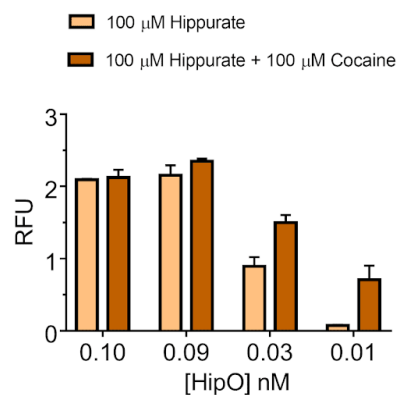
Supplementary Figure S9.12. Further characterization of HipO enzyme (hippurate transforming enzyme) at lower concentrations of the enzyme and 100 μM hippurate. HipO enzyme which for its weight led to higher signals than predicted, needed to be further characterized at concentrations lower than the minimum concentration used for the weighted metabolic circuits (0.1 nM). For this characterization, this figure shows the effect of 100 μM hippurate input alone and its additive effect when coupled with 100 μM cocaine at the weight (CocE enzyme concentration) of 0.1 nM. All data are the mean and the error bars are the standard deviation of normalized values from measurements taken from two or three independent cell-free reactions on the same day. (RFU: Relative Fluorescence Unit).
