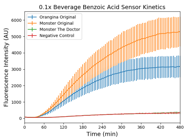
Supplementary Figure S8.8. Time course of the benzoic biosensor response to 1x and 0.1x beverages. Kinetics of sfGFP expression at 37°C using our optimized benzoic acid biosensor to detect benzoates in commercial beverages. The top panel depicts kinetics in response to addition of 2 \mu L of unaltered beverage to a 20 \mu L cell-free reaction. The bottom panel depicts kinetics after the samples were first diluted 1:10 in water before being added to the reaction. ‘Orangina Original’ and ‘Monster Original’ include sodium benzoate and benzoic acid, respectively, in their list of ingredients. ‘Monster The Doctor’ lists no benzoates in the ingredients. Water was used in place of the beverage for the negative control. Data depict the mean of three experiments conducted on three different days and error bars represent the standard deviation. Fluorescence intensity y-axis scale was adjusted for the weaker signal dilution experiment to enable adequate visualization of the kinetics.
