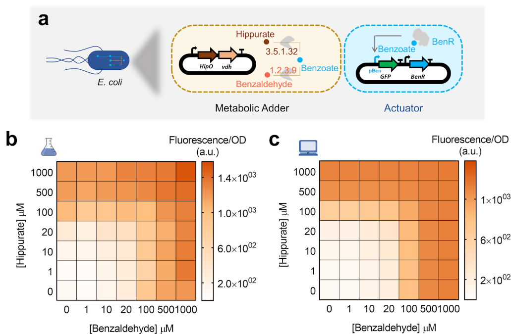
Figure 9.2. Whole-cell metabolic adder of hippurate and benzaldehyde. (a) Hippurate and benzaldehyde transducers are combined to build a metabolic adder producing a common output, benzoate, which is reported through the benzoate actuator. The genes encoding the enzymes are
