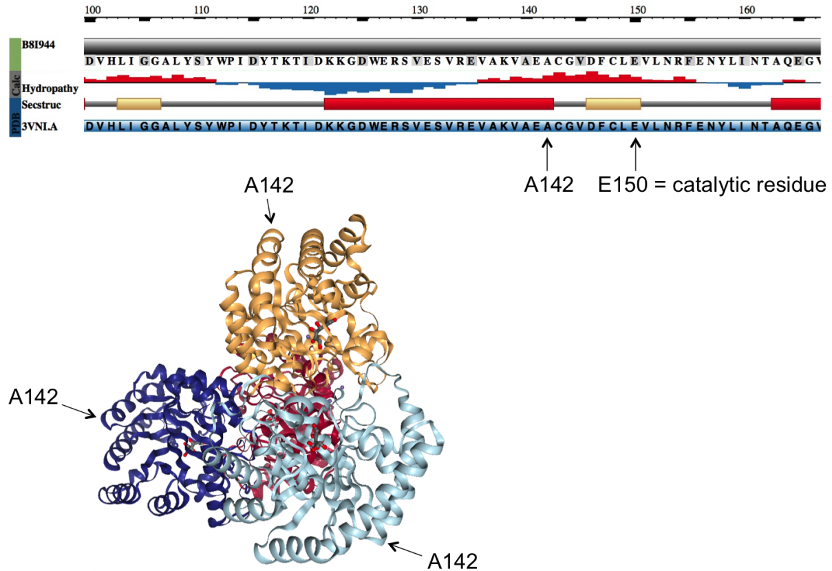
Supplementary Figure S5.4. Structure of C. cellulolyticum DPEase. (A) Protein feature view of PDB entry 3VNI.A mapped to the UniProt sequence B8I944. (B) Ribbon representation of PDB entry 3VNI.A (image created with NGL Viewer [340]). The catalytic glutamate (E150) is indicated as well as the alanine residue (A142) that was found mutated into an asparagine upon screening of a random mutant library for DPEase mutants for potentially improved catalytic efficiency.
