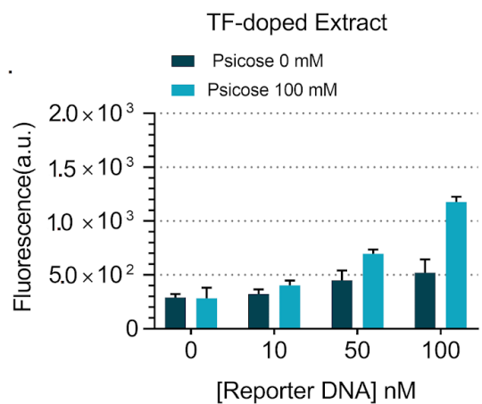
Supplementary Figure S6.3 (matches with Figure 6.2d). Fluorescence level for TF-doped extract with and without psicose. The fluorescence fold change plotted in Figure 6.2d is the ratio between two bars presented in this figure for different concentrations of reporter DNA. The data and error bars are the mean and standard deviation of three measurements from three independent reaction done in the same day using the same lysate and maxiprepped plasmids.
