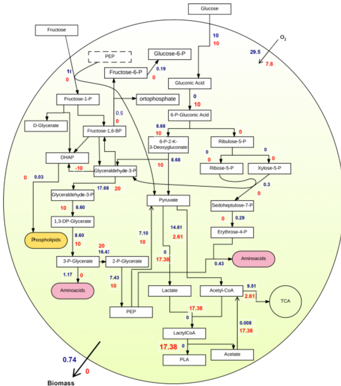
Figure 4.2. Schematic representation of the central metabolism with PLA pathway, using glucose as substrate. In this flux distribution, glucose was defined as the carbon source. The blue flux values are associated with Biomass optimized FBA and the red flux values are associated with PLA production FBA. These two FBAs were done in independent experiments.
