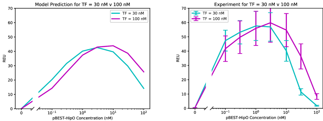
Supplementary Figure S8.5. Model-predicted shift in HipO concentration for peak biosensor signal at high concentrations of TF plasmid and inducer. Increasing TF plasmid concentration results in a right-shift of HipO plasmid concentration for optimal performance. Left panel: Model calculations for sfGFP output for a range of pBEST-HipO concentrations for TF plasmid concentrations at 30 nM and 100 nM. Right panel: Experimental results to examine if the same right-shift could be seen experimentally. Results are the mean from three experiments on three different days and error bars represent the standard deviation. For all experiments and model calculations, reporter plasmid concentration was fixed at 100 nM and a hippurate inducer concentration of 1000 \mu M was used. All fluorescence values have relative expression units (REU) compared to the four hour level for 100 pM of a strong, constitutive sfGFP-producing plasmid.
