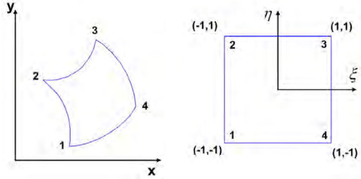
Figure 5.2 – Global and local elements
