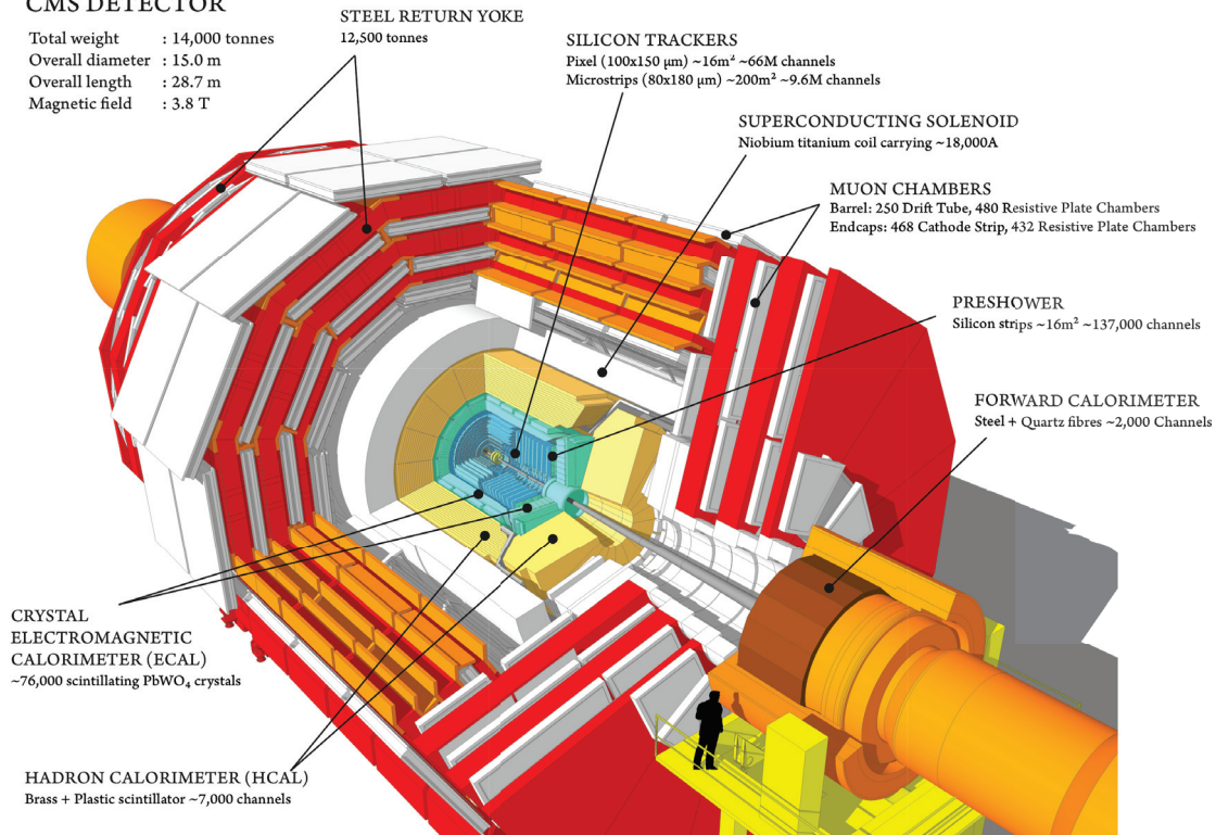
Figure 2.2: Illustration of the CMS detector and its concentric layers of subdetectors along with the superconducting solenoid and the steel return yoke.
