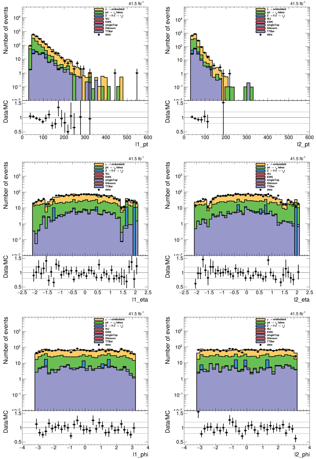
Figure B.2: Comparison of the distributions obtained from the estimation methods and observed data for the leading ( l_1 ) and sub-leading ( l_2 ) selected \tau_h kinematic variables in the b -tag category.
