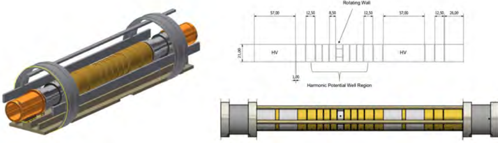
Figure 6.10 GBAR antiproton trap electrodes.
