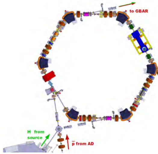
Figure 5.31 The 30.4 m circumference ELENA synchrotron ring. ELENA receives 100 keV H^- beam from a source ( bottom left ) or 5.3 MeV antiproton beam from the AD ( bottom ) and circulates clockwise. The beams are extracted from the LNE50 beam line ( top right ).
