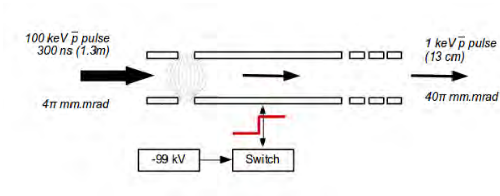
Figure 2.12 Principle scheme of the GBAR decelerator.
