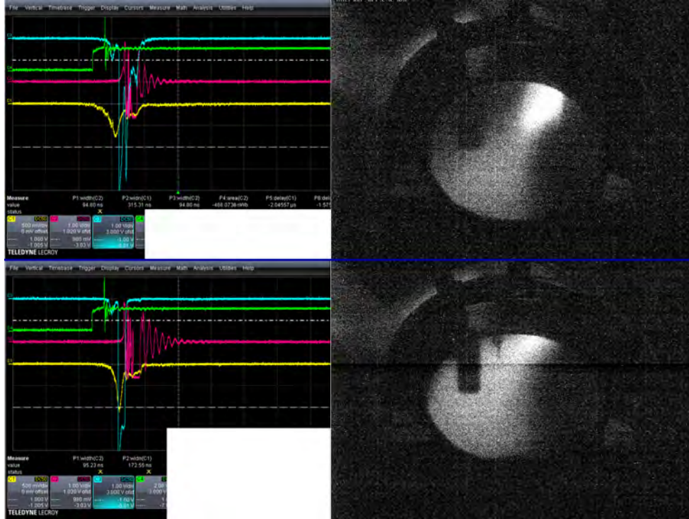
Figure 5.38 (right) MCP/PS image of the antiproton beam; (left) oscilloscope traces showing the HV-switch trigger (green), MCP charge signal (red), upstream scintillator (blue) and downstream scintillator (yellow). Top panel is with no Einzel-lens voltage and bottom with 20 kV. The shadow of the Ps support (see Figure-5.37) is visible.
