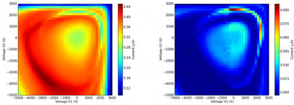
Figure 5.22 Beam current as measured on the hat-shaped mask ( left ) and in the Faraday Cup ( right ) for a 2- keV proton beam. The color is proportional to the current value. The electrode are identified as #1 and #2 corresponding respectively to the first and second lens.
