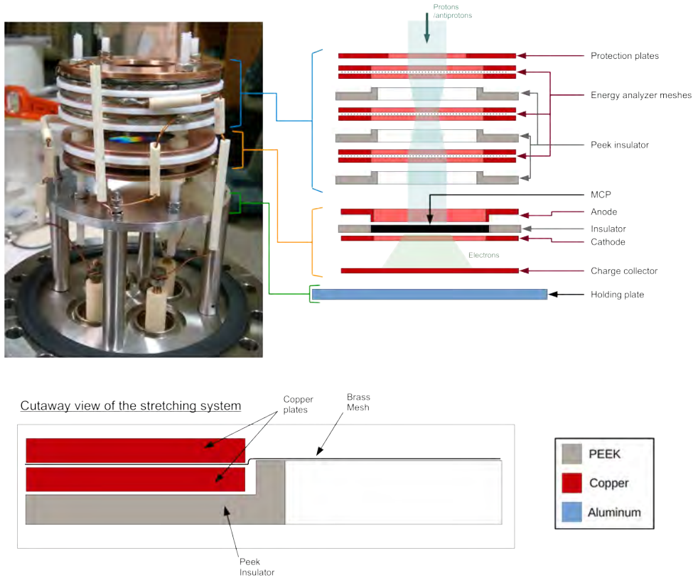
Figure 5.27 Schematic and picture of the improved energy analyzer.
