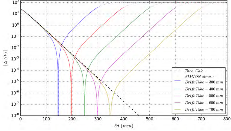
Figure 3.5 Evaluation of the axial potential variation along the pulsed drift tube with respect to the distance \delta d from the edge of the drift tube. (dashed line) - Theoretical estimation for a R = 50 mm semi-infinite cylinder initially polarized at V_{PDT} = -99 kV. (solid lines) - Corresponding simulations of the potential spread for 5 different sizes of drift tubes (finite length, R = 50 mm) obtained with SIMION.
