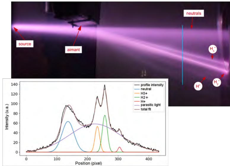
Figure 6.15 Photograph of the separation of the different species extracted from the TES35 source by a magnet placed at the nearest beam during preliminary tests conducted by Polygon Physics. The insert represents the profile of the light intensity of the beam picture along the blue line. Data from the Polygon Physics.
