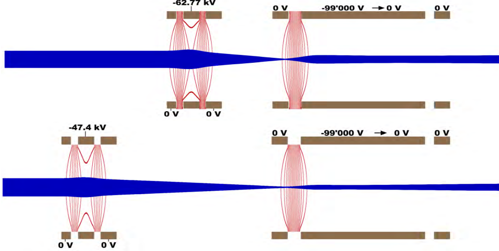
Figure 3.10 Comparison of simulated telescopic systems for a 1\text{ keV} deceleration. The apparatus is composed of an Einzel lens and a pulsed drift tube. The initial beam is taken homogeneous over a radius R = 10\text{ mm} and parallel to the optical axis with an energy of exactly 100\text{ keV} . The red lines correspond to the equipotentials with a 5\text{ kV} step. (Top) - Distance between the Einzel lens and the drift tube L = 500\text{ mm} . The spot of the emerging beam is 8\text{ mm} . (Bottom) - Distance between the Einzel lens and the drift tube L = 1000\text{ mm} . The spot of the emerging beam is 4\text{ mm} .
