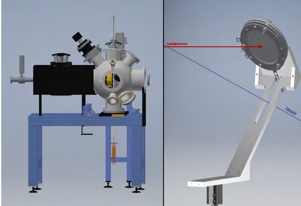
Figure 5.37 ( left ) Reaction chamber showing the end of the positron line (positrons arrive from the left) and the MCP mounted inside (in its retracted position – the antiprotons arrive from the front). ( right ) detail of the MCP mounting showing the angle required for passage of the laser beam for exciting the Ps cloud.
