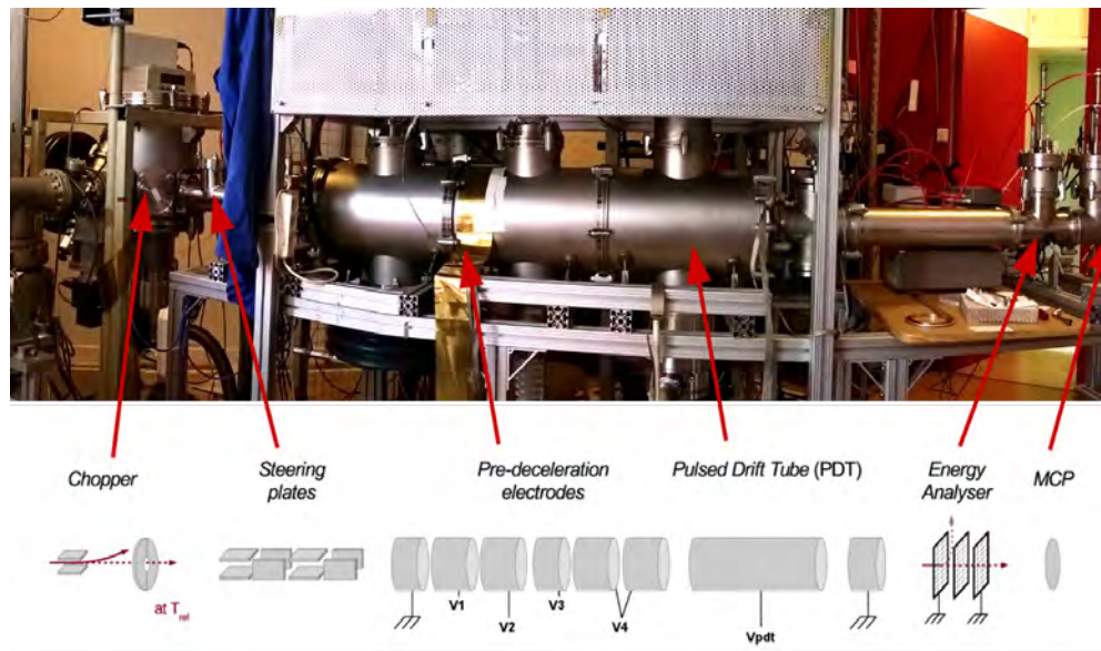
Figure 5.1 Picture and schematic of the prototype off-line decelerator test bench as installed in Orsay from 01/2016 to 08/2016. The ion beam is flying from left to right over 3 m .
