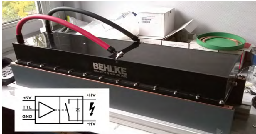
Figure 5.9 Picture of the BEHLKE HTS 1501-20-LC2 single pole, single throw (very) high voltage switch. The switch is presented mounted on insulated plastic supports.
