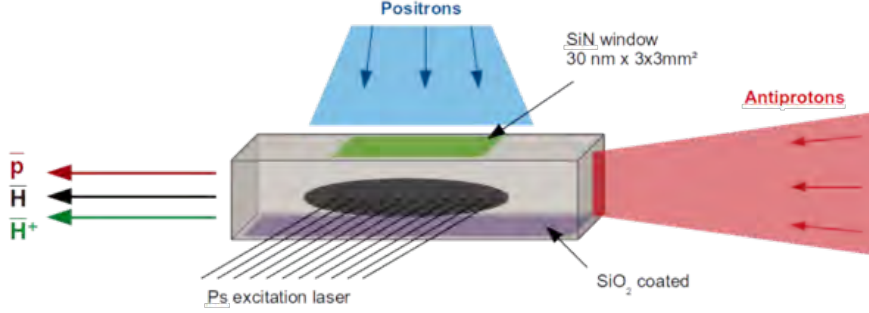
Figure 2.7 Sketch of the \bar{p} - Ps interaction region.
