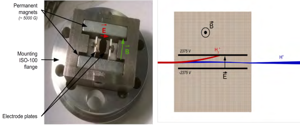
Figure 5.6 ( Left ) - Picture of the Wien filter on its mounting flange. ( Right ) - SIMION simulation of the Wien filter for a 10 \text{ keV } H^+/H_2^+ beam example. The initial beam is here 2.5 \text{ mm} -large and parallel.
