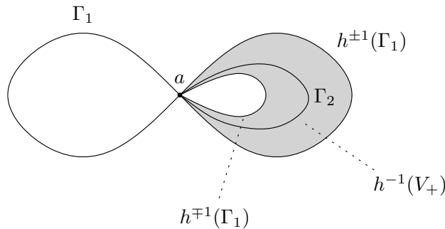
Figure 5.5 – The construction of the line \Gamma_2
