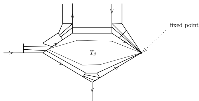
Figure 5.25 – The foliation in T_\beta when \beta \in B is a half-plane with an initial vertex
