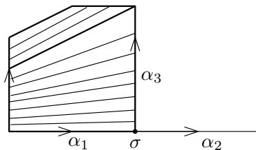
Figure 5.18 – The case where \alpha_2 is singular and \alpha_3 is regular
