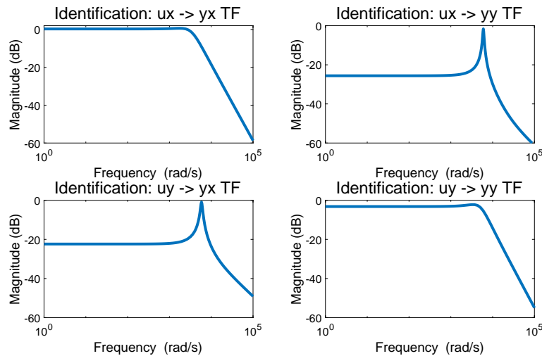
Figure 4.22: Scanning MODE identification: Transfer functions
