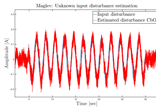
Figure 5.12: Real-time: sinusoidal input disturbance estimation
