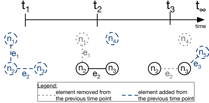
Figure 7.2: Evolution of a temporal graph over time
