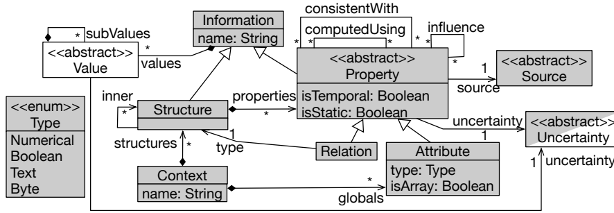
Figure 7.6: Excerpt of the context metamodel
