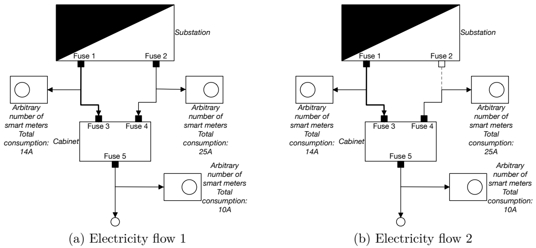
Figure 3.1: Two different electric flows for a same grid topology
