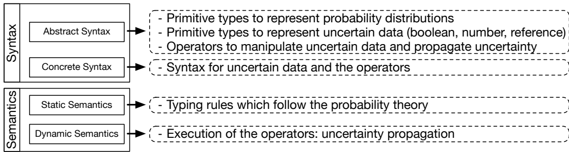
Figure 6.1: Impact of having uncertainty as a first-class language citizen on a language
