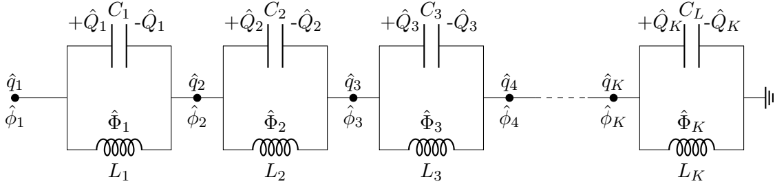
Figure A.1: Calderira-Leggett model of an impedance. These resonators can be described by two sets of variables, the charge \hat{q}_k and flux \hat{\phi}_k at the node k or the flux \hat{\Phi}_k through the inductor k and the charge \hat{Q}_k of the capacitor k .
