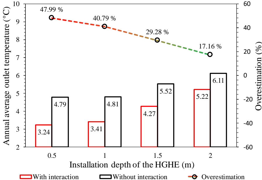
Figure VI.17. Comparison between the annual average fluid outlet temperatures with and without the atmosphere-soil interaction
