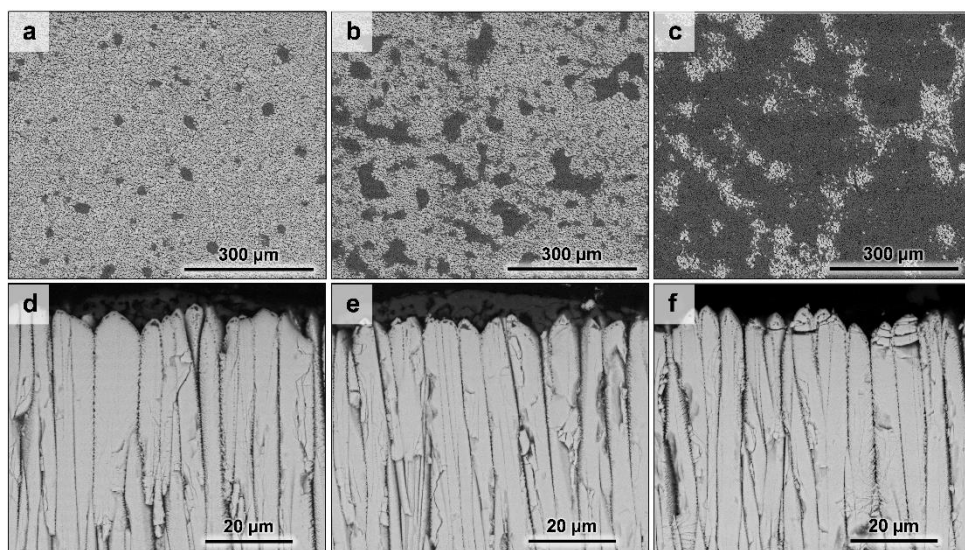
Fig. 4 – SEM micrographs of the co-stabilised ErYSZ coating with CMAS deposits of (a, d) 0.25, (b, e) 1 and (c, f) 5 mg.cm -2 annealed in air at 1250°C for 1h.
