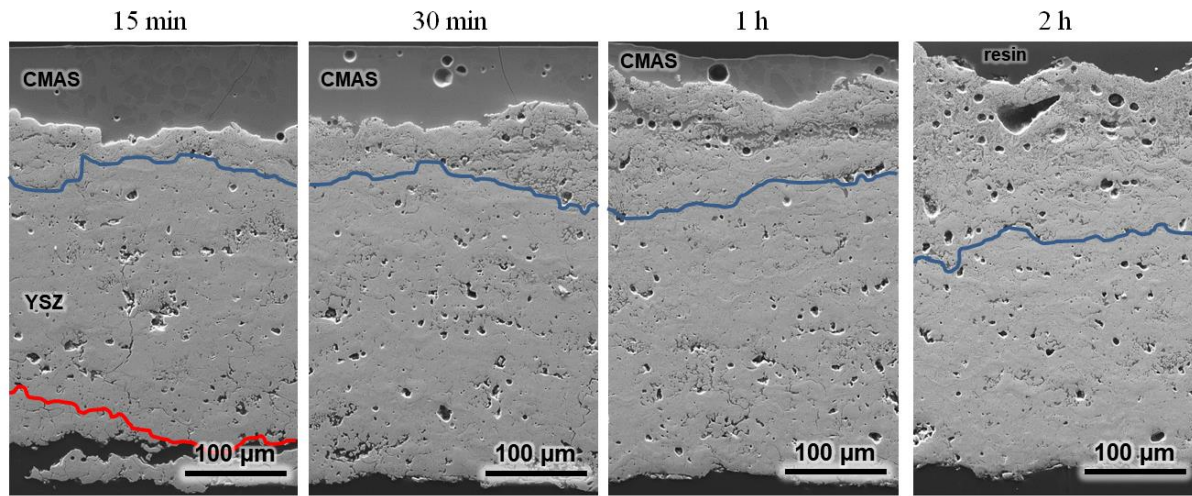
Figure II.5 – Plasma-sprayed coatings with 20 mg.cm -2 of CMAS after exposure to 1250°C.
