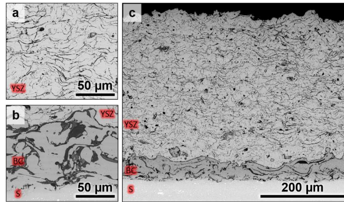
Figure 4 –Cross-sections of the INJ_APS sample with a and b being higher magnifications of the ceramic microstructure and the bond coating, respectively.
