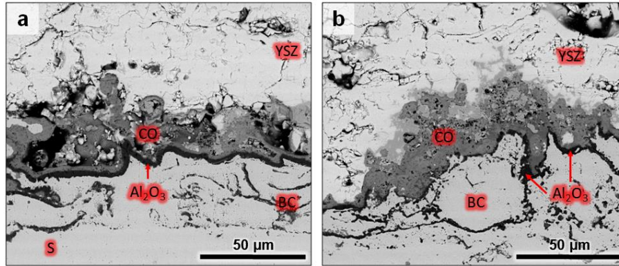
NB: YSZ = ceramic; BC = bond coating; S = substrate; CO = complex (Ni, Cr, Al) oxides; Figure 9 – SEM cross-section at the interface between the bond and ceramic coatings after exposure at 1100°C in air for (a) 150h in isothermal conditions and (b) 100 1-hour cycles.
