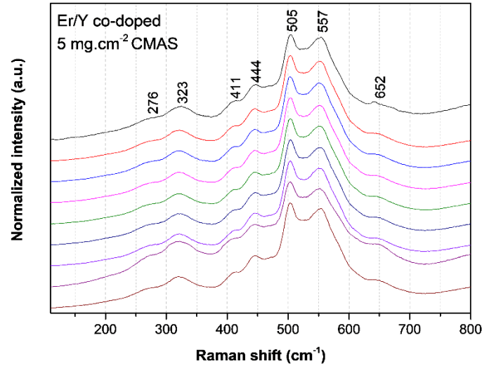
Fig. 7 – Raman spectra in the cross sections of the ErYSZ coating annealed in air at 1250^\circ\text{C} for 1h with 5 \text{ mg.cm}^{-2} CMAS deposit.
