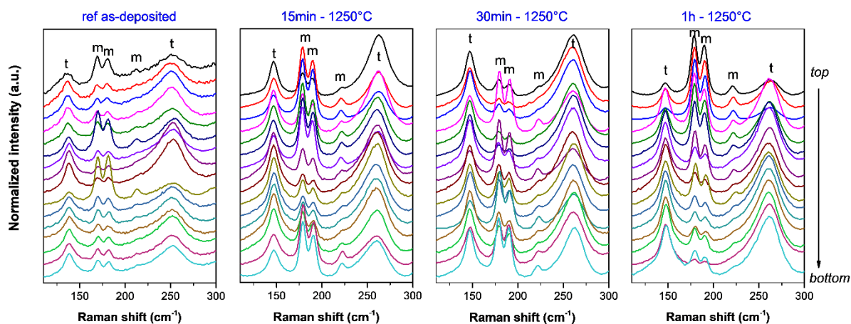
Figure 3 – Raman local spot analysis of plasma-sprayed YSZ coatings annealed at 1250^\circ\text{C} for different times with CMAS deposits of 20 \text{ mg.cm}^{-2} .
