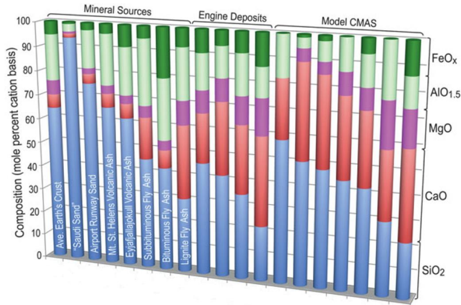
Figure I.25 – Concentration of predominant oxides in the composition of calcium-magnesium alumino-silicates, grouped by examples of sources of siliceous debris, compositions reported for actual deposits in engines, and model compositions used in laboratory investigations of the problem. [71]
