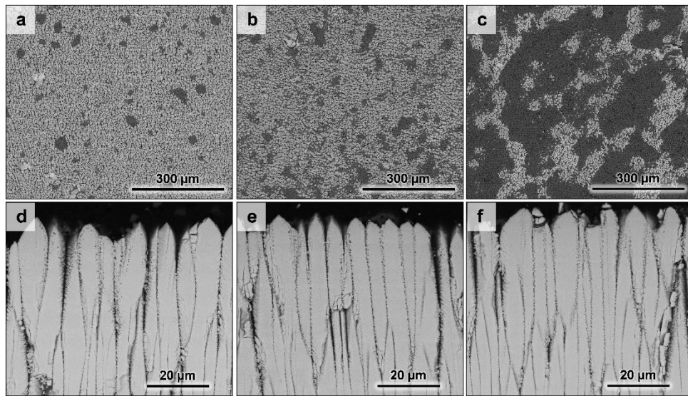
Fig. 3 – SEM micrographs of the standard 8YSZ coating with CMAS deposits of (a, d) 0.25, (b, e) 1 and (c, f) 5 mg.cm -2 annealed in air at 1250°C for 1h.
