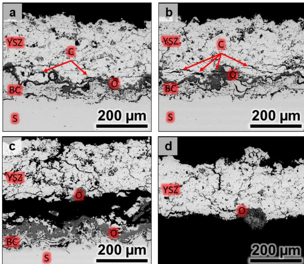
NB: YSZ = ceramic; BC = bond coating; S = substrate; O = oxides; OGB = oxidized grain boundaries; C = cracks Figure 10 - SEM micrographs of the cross-sections of the IN_APS samples after cyclic exposure (1h-cycles at 1100°C in air) for (a) 50, (b) 150, (c) 250 and (d) 500 h.
