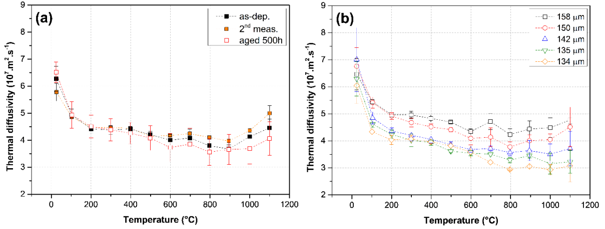
Fig. 5 – a) Thermal diffusivity as a function of the temperature for the 8YSZ standard coatings in the as-deposited conditions, pre-sintered during the first measurement and aged in air at 1100^{\circ}\text{C} for 500h and b) details of the 5 samples after ageing.
