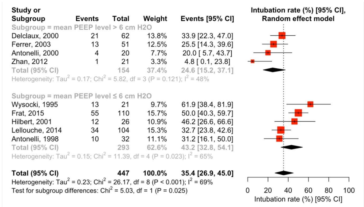
Figure 4. Forrest plot comparing the incidence of intubation rates in patients with de novo acute hypoxemic respiratory failure treated with noninvasive ventilation using high or low positive end-expiratory pressure levels.
