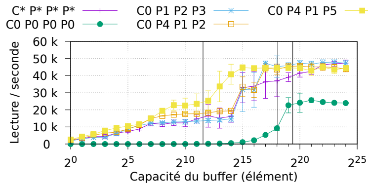
(a) : Attente active
