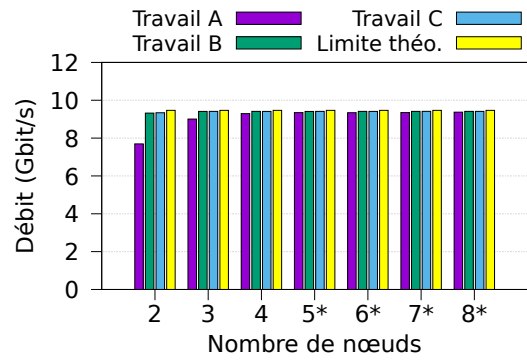
(b) : one-to-many
