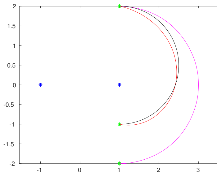
Fig. 5.32: \Sigma := \{M(-1, 0), N(1, 0)\} : red curve and magenta curve are two optimal trajectories, black curve (a half circle) is not a optimal trajectory.
