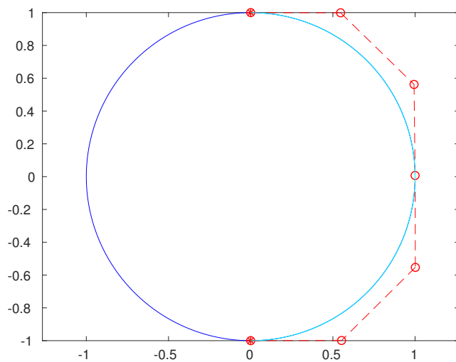
Fig. 5.15: Step 4 in Example 5.5: the local minimum \tilde{\gamma}_2 \in B_{2,3} of F|_{B_{2,3}} from the initial curve \gamma_2 \in B_{2,3} .
