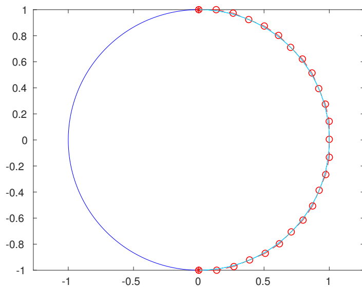
Fig. 5.26: Step 15 in Example 5.5: split at the seventh piece and reparametrize \gamma_7 \in B_{7,3} to become \gamma_8 \in B_{8,3} .
