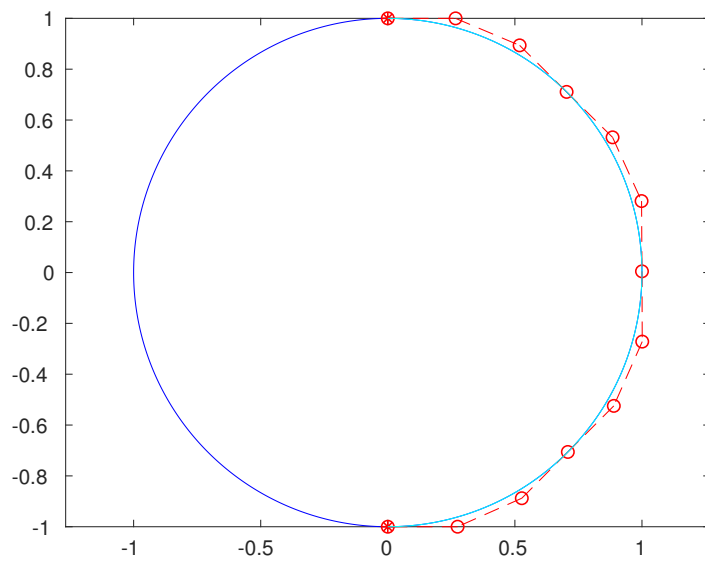
Fig. 5.19: Step 8 in Example 5.5: the local minimum \tilde{\gamma}_4 \in B_{4,3} of F|_{B_{4,3}} from the initial curve \gamma_4 \in B_{4,3} .
