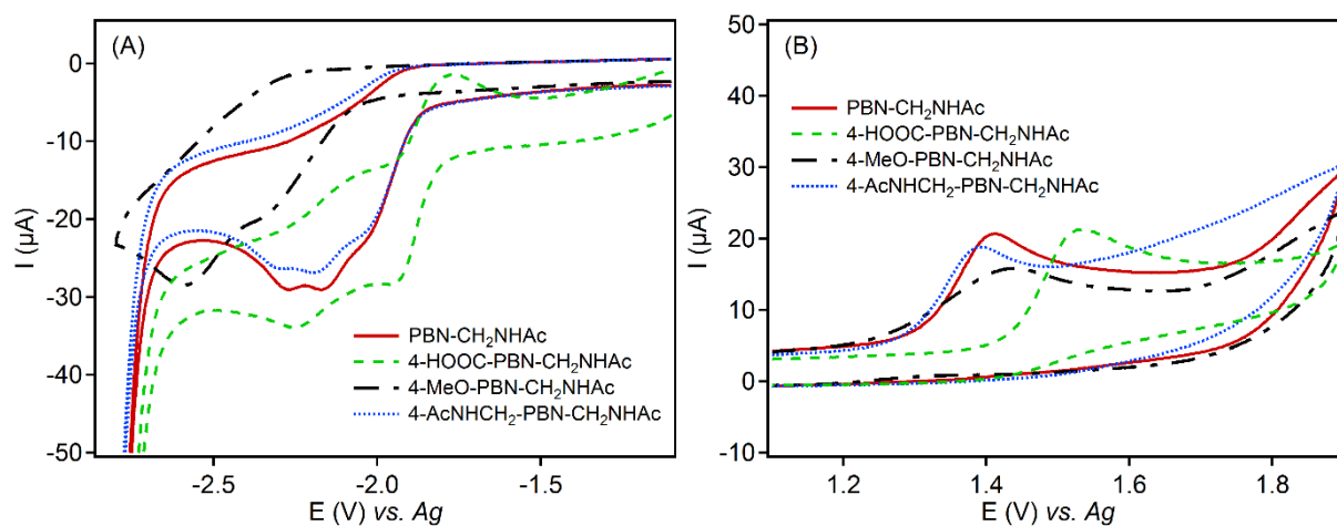
Figure S2. Cyclic voltammograms of X-PBN-CH 2 NHAc derivatives in acetonitrile containing 0.1 M of TBAP at a GC electrode, potential scan rate v = 0.1 V/s: (A) reduction and (B) oxidation.
