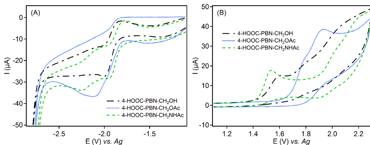
Figure S1. Cyclic voltammograms of 4-HOOC-PBN-CH 2 Y derivatives in acetonitrile containing 0.1 M of TBAP at a GC electrode, potential scan rate v = 0.1 V/s: (A) reduction and (B) oxidation.
