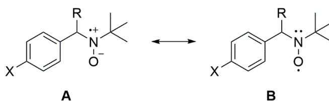
Scheme 15. Resonance structures for 4-X-PBN-R adducts.
