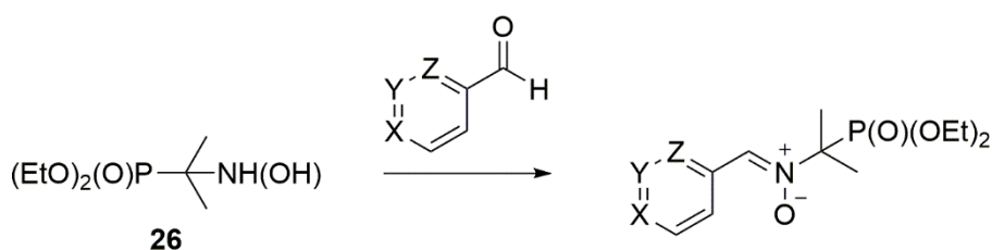
Scheme 17. Improved synthetic route of PPN derivatives.
