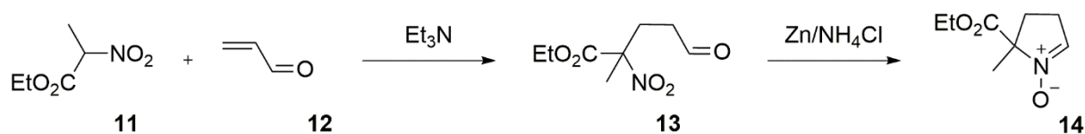
Scheme 12. Synthesis of EMPO.
