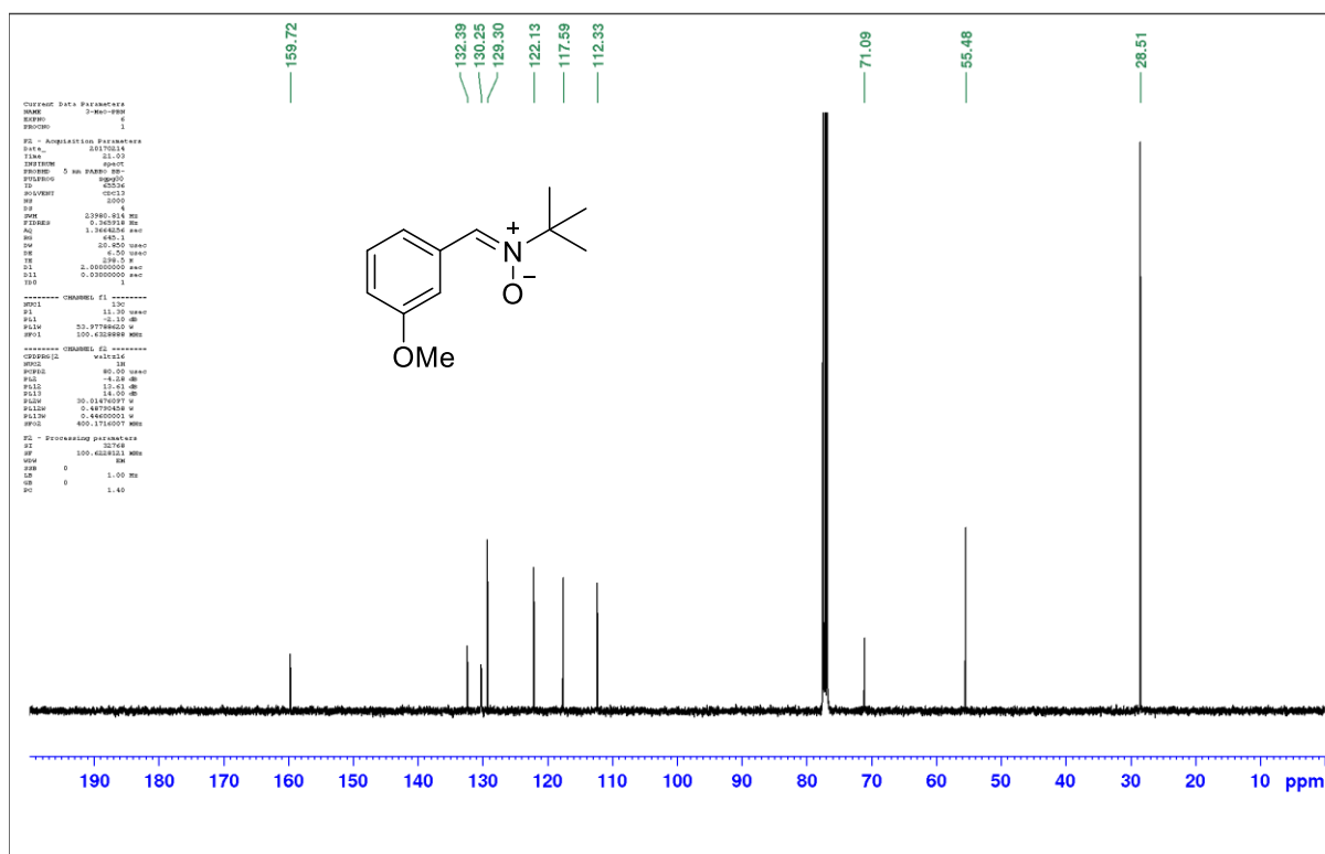
Figure S4. ^{13}\text{C} NMR spectrum of compound 2 in \text{CDCl}_3 .
