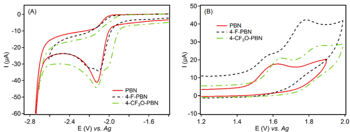
Figure S2. Cyclic voltammograms of PBN, 4-F-PBN and 4-CF 3 O-PBN, reduction (A) and oxidation (B) in acetonitrile containing 0.1 M of TBAB at a GC electrode, potential scan rate v = 0.1 V/s.
